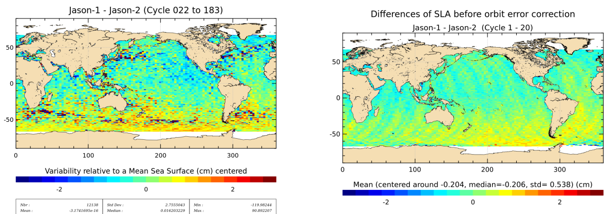
FIGURE 19 – Jason-1 – Jason-2 SLA differences averaged over Jason-2 period from cycle 022 until cycle 183 (left), and for tandem phase (cycle 001 to 020) (right).
