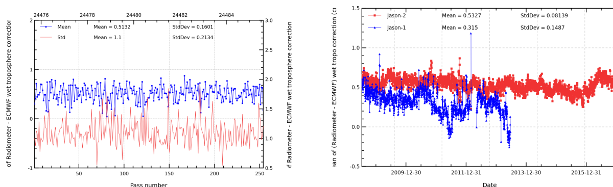
FIGURE 11 – Pass monitoring of wet troposphere differences between radiometer and ECMWF model for Jason-2 cycle 314 (left) and daily monitoring of wet troposphere differences between radiometer and ECMWF model (right).
