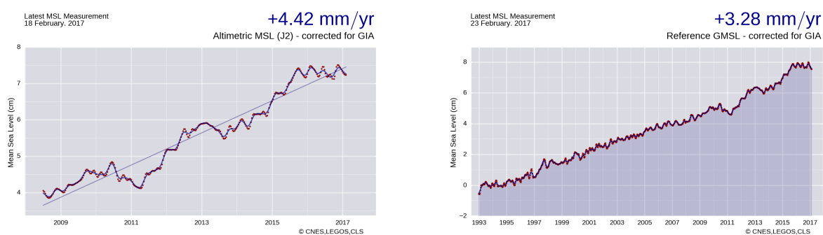
FIGURE 21 – Global MSL on Jason-2 mission (left) and with reference missions from 1993 onwards (right).
