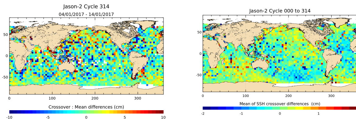
FIGURE 12 – Mean SSH at crossovers for cycle 314 (left) and over the whole Jason-2 period (right).
