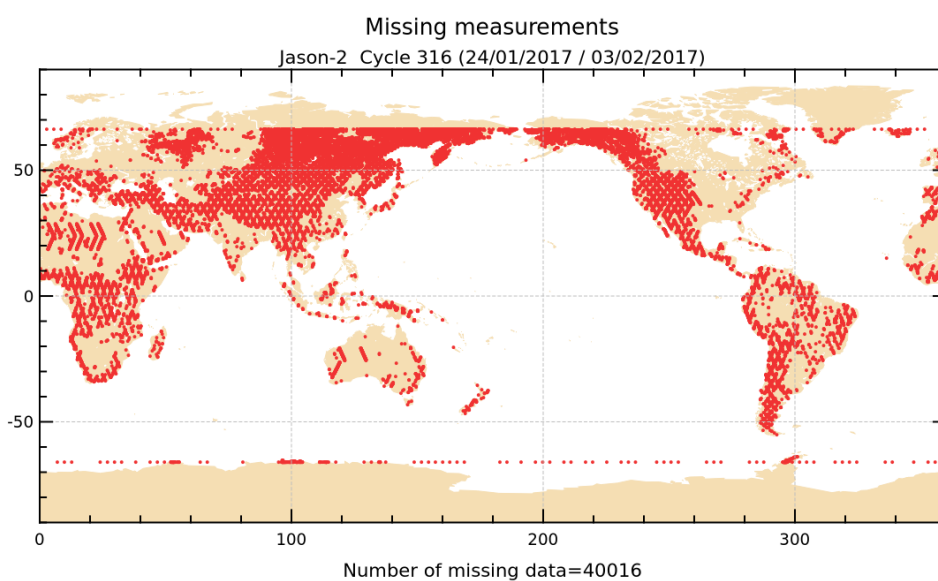
FIGURE 1 – Missing measurements for cycle 316.
