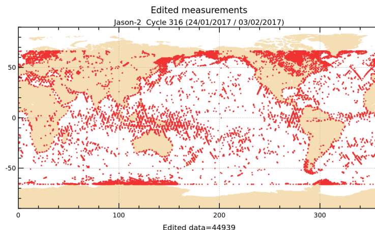
FIGURE 2 – Edited measurements for cycle 316.
