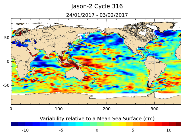
FIGURE 17 – Sea level anomaly relative to MSS for cycle 316.
