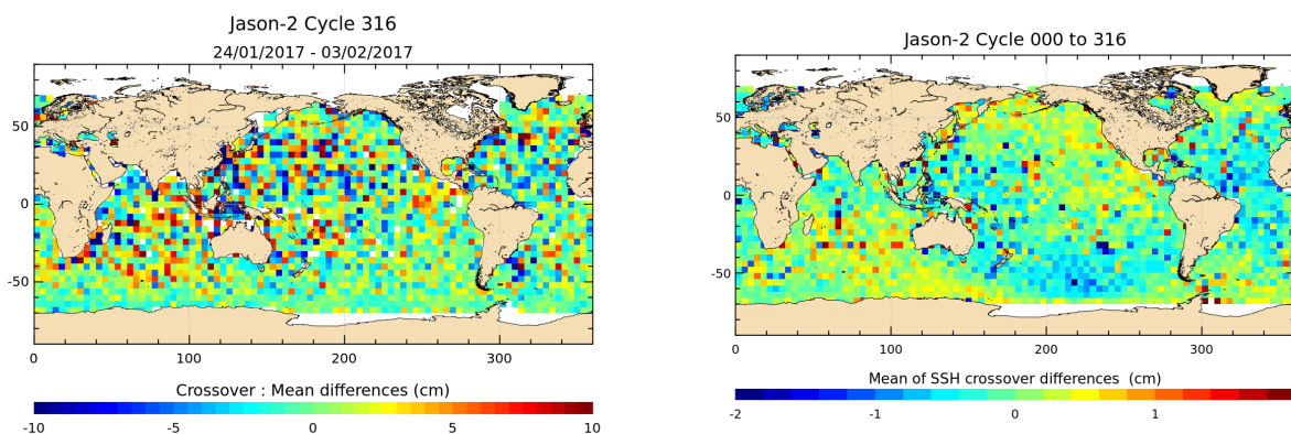
FIGURE 12 – Mean SSH at crossovers for cycle 316 (left) and over the whole Jason-2 period (right).
