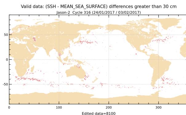
FIGURE 18 – Differences higher than a 30 cm threshold for cycle 316.
