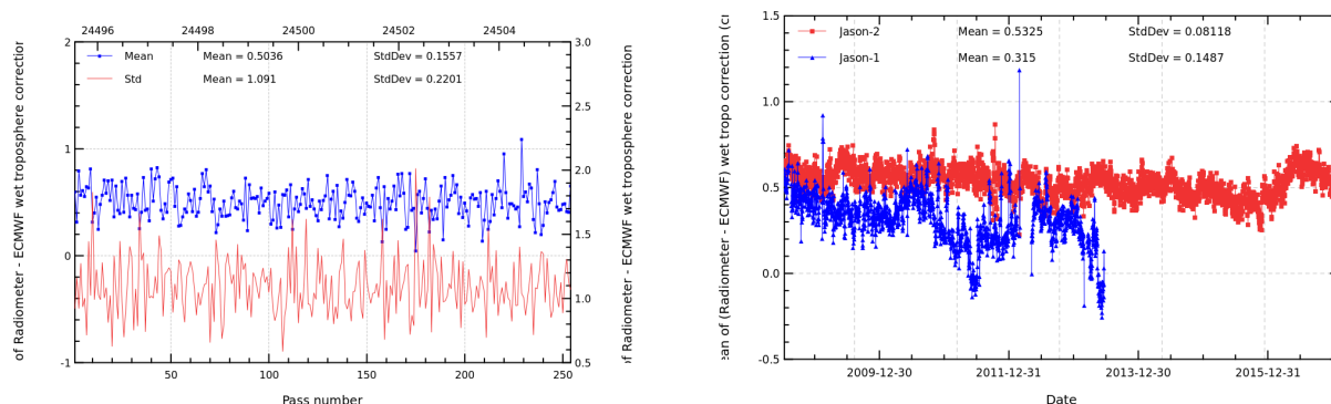
FIGURE 11 – Pass monitoring of wet troposphere differences between radiometer and ECMWF model for Jason-2 cycle 316 (left) and daily monitoring of wet troposphere differences between radiometer and ECMWF model (right).
