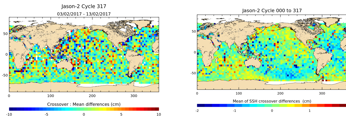
FIGURE 12 – Mean SSH at crossovers for cycle 317 (left) and over the whole Jason-2 period (right).
