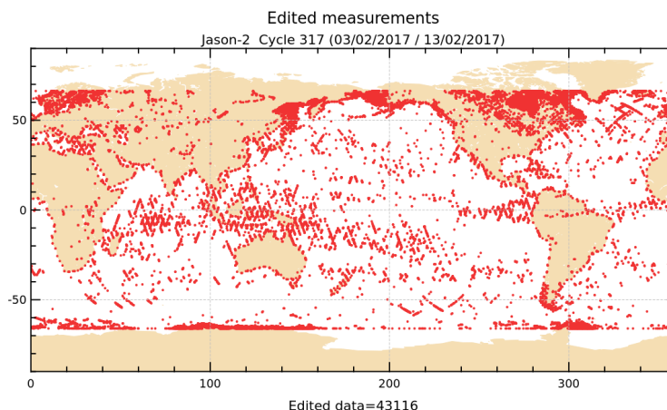
FIGURE 2 – Edited measurements for cycle 317.
