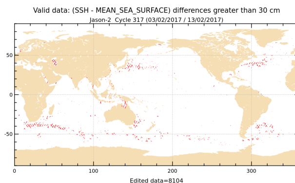
FIGURE 18 – Differences higher than a 30 cm threshold for cycle 317.
