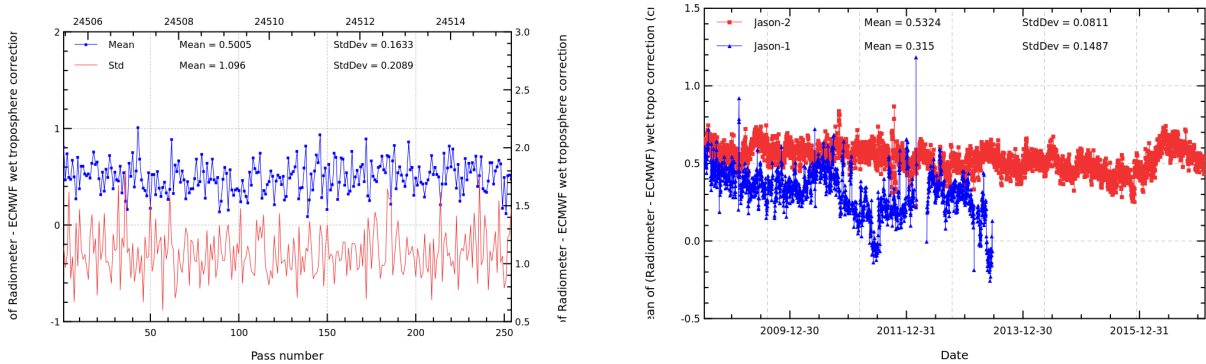
FIGURE 11 – Pass monitoring of wet troposphere differences between radiometer and ECMWF model for Jason-2 cycle 317 (left) and daily monitoring of wet troposphere differences between radiometer and ECMWF model (right).
