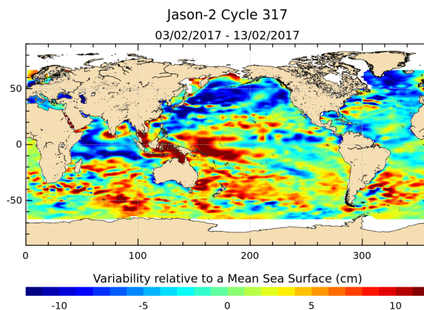
FIGURE 17 – Sea level anomaly relative to MSS for cycle 317.
