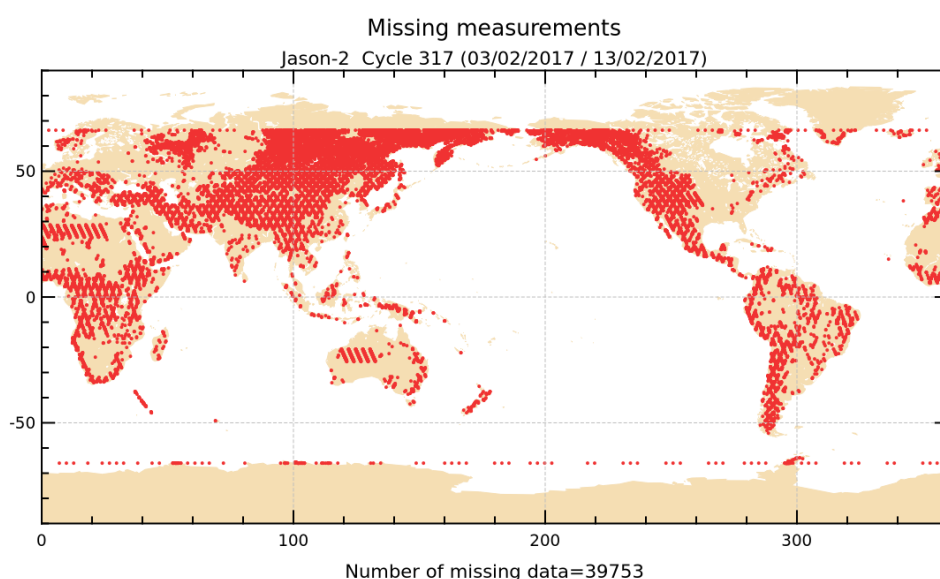
FIGURE 1 – Missing measurements for cycle 317.
