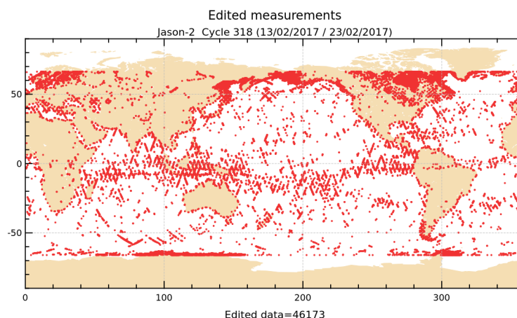
FIGURE 2 – Edited measurements for cycle 318.
