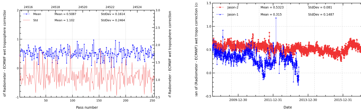
FIGURE 11 – Pass monitoring of wet troposphere differences between radiometer and ECMWF model for Jason-2 cycle 318 (left) and daily monitoring of wet troposphere differences between radiometer and ECMWF model (right).
