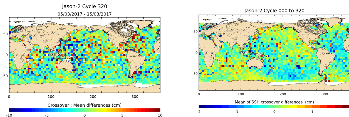
FIGURE 12 – Mean SSH at crossovers for cycle 320 (left) and over the whole Jason-2 period (right).
