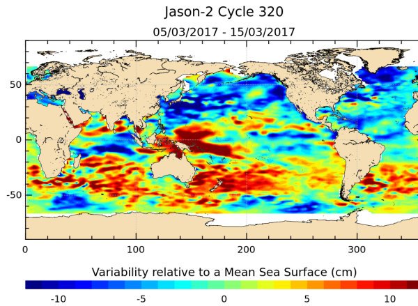
FIGURE 17 – Sea level anomaly relative to MSS for cycle 320.
