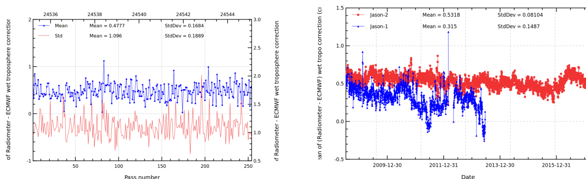
FIGURE 11 – Pass monitoring of wet troposphere differences between radiometer and ECMWF model for Jason-2 cycle 320 (left) and daily monitoring of wet troposphere differences between radiometer and ECMWF model (right).
