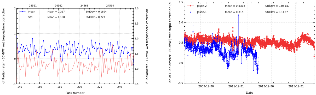
FIGURE 11 – Pass monitoring of wet troposphere differences between radiometer and ECMWF model for Jason-2 cycle 322 (left) and daily monitoring of wet troposphere differences between radiometer and ECMWF model (right).
