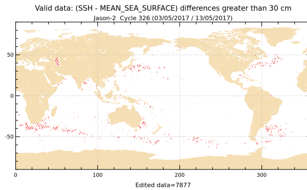
FIGURE 18 – Differences higher than a 30 cm threshold for cycle 326.
