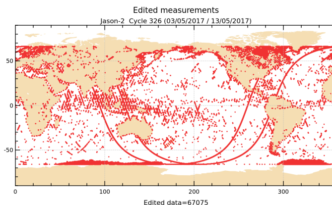
FIGURE 2 – Edited measurements for cycle 326.
