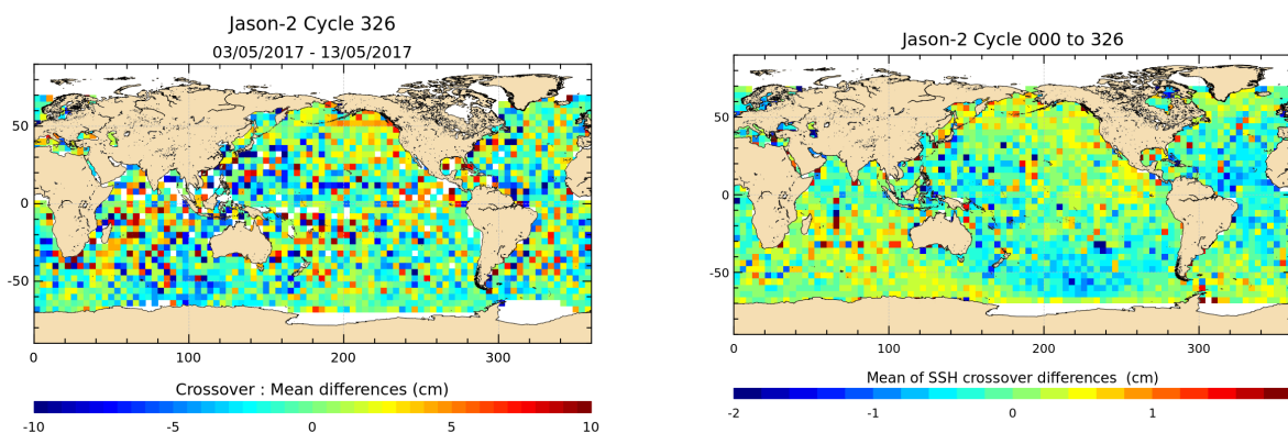
FIGURE 12 – Mean SSH at crossovers for cycle 326 (left) and over the whole Jason-2 period (right).
