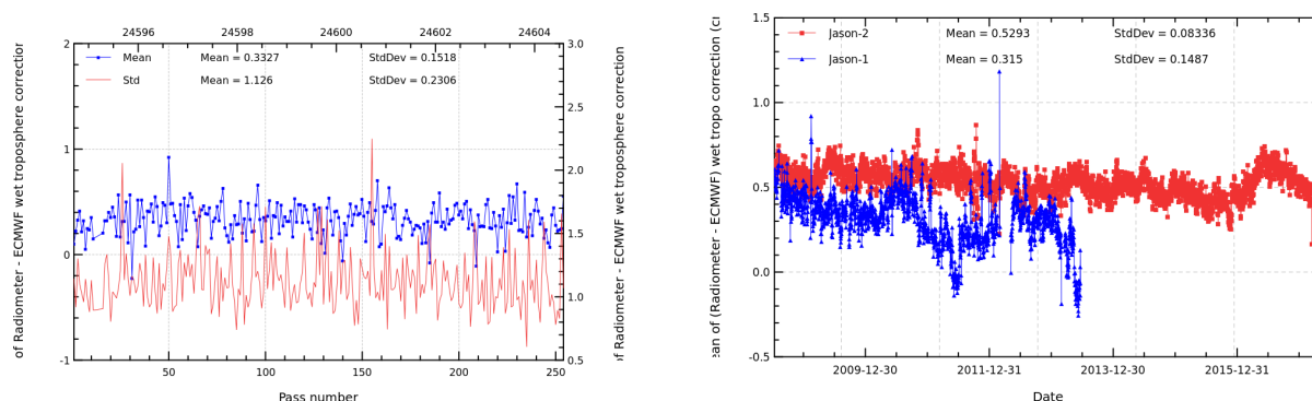
FIGURE 11 – Pass monitoring of wet troposphere differences between radiometer and ECMWF model for Jason-2 cycle 326 (left) and daily monitoring of wet troposphere differences between radiometer and ECMWF model (right).
