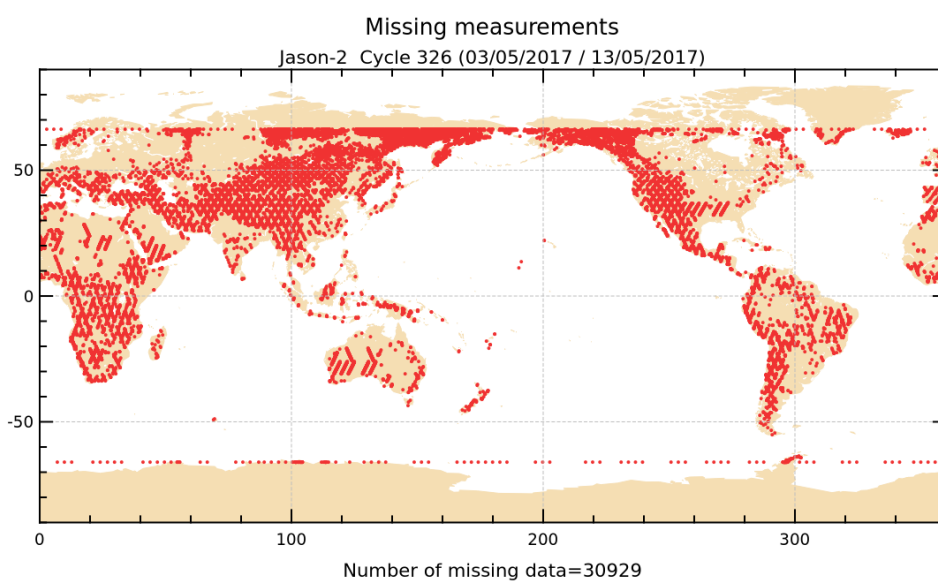
FIGURE 1 – Missing measurements for cycle 326.
