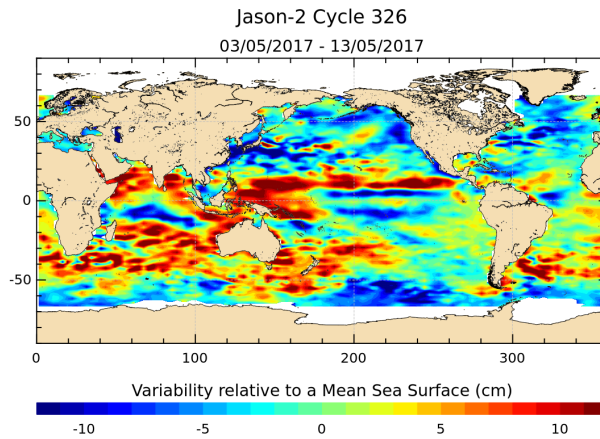
FIGURE 17 – Sea level anomaly relative to MSS for cycle 326.
