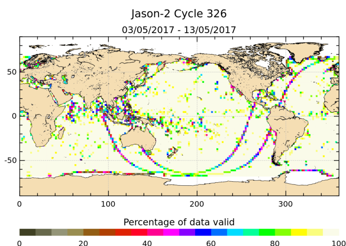
FIGURE 3 – Percentage of valid measurements for cycle 326.
