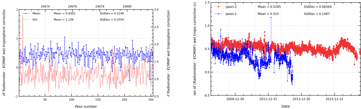
FIGURE 11 – Pass monitoring of wet troposphere differences between radiometer and ECMWF model for Jason-2 cycle 501 (left) and daily monitoring of wet troposphere differences between radiometer and ECMWF model (right).
