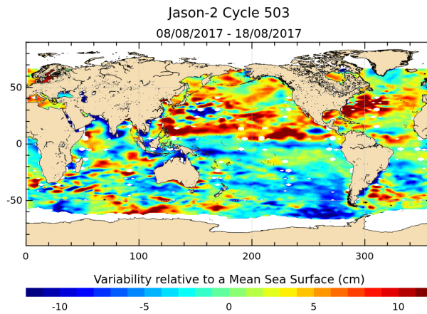
FIGURE 17 – Sea level anomaly relative to MSS for cycle 503.
