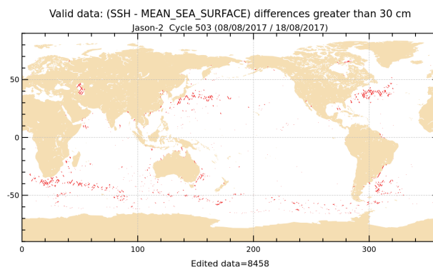
FIGURE 17 – Sea level anomaly relative to MSS for cycle 503.
