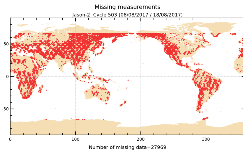
FIGURE 1 – Missing measurements for cycle 503.
