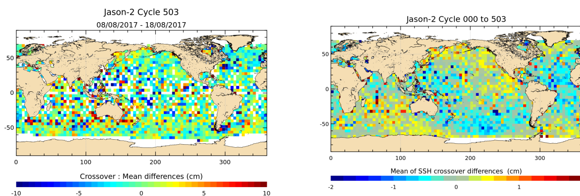
FIGURE 12 – Mean SSH at crossovers for cycle 503 (left) and over the whole Jason-2 period (right).
