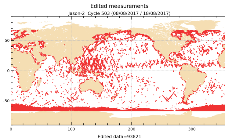
FIGURE 2 – Edited measurements for cycle 503.
