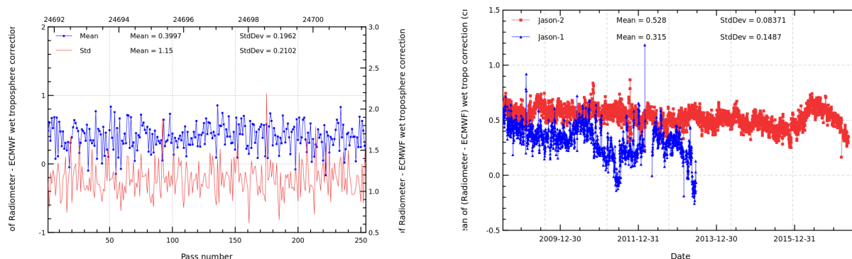
FIGURE 11 – Pass monitoring of wet troposphere differences between radiometer and ECMWF model for Jason-2 cycle 503 (left) and daily monitoring of wet troposphere differences between radiometer and ECMWF model (right).
