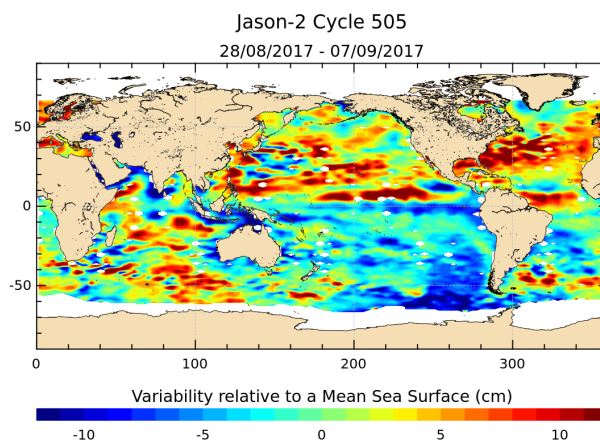
FIGURE 17 – Sea level anomaly relative to MSS for cycle 505.
