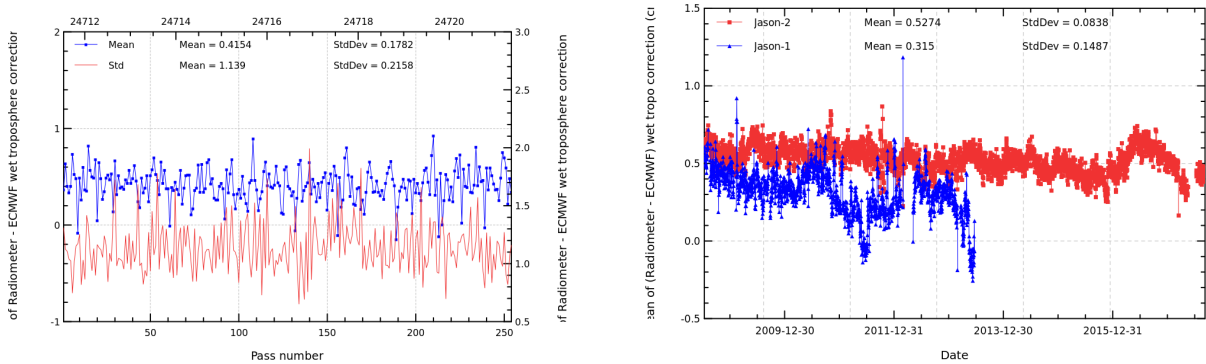
FIGURE 11 – Pass monitoring of wet troposphere differences between radiometer and ECMWF model for Jason-2 cycle 505 (left) and daily monitoring of wet troposphere differences between radiometer and ECMWF model (right).
