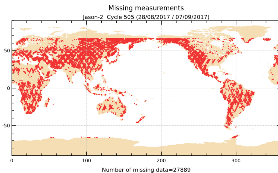
FIGURE 1 – Missing measurements for cycle 505.
