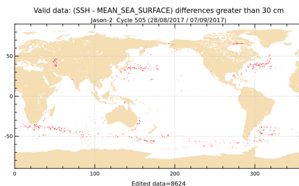
FIGURE 17 – Sea level anomaly relative to MSS for cycle 505.
