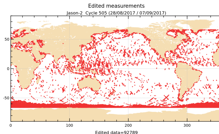
FIGURE 2 – Edited measurements for cycle 505.
