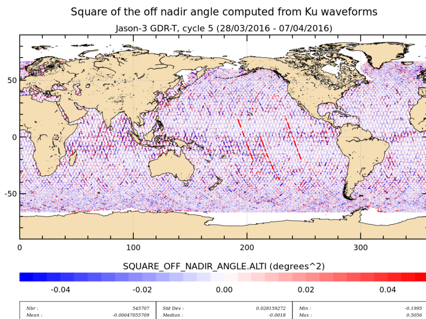
FIGURE 4 – Apparent squared mispointing from waveforms for cycle 005.
