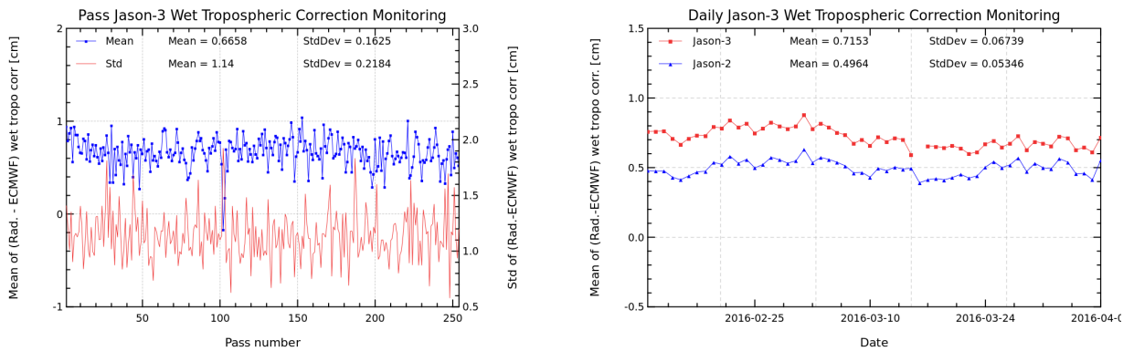
FIGURE 12 – Pass monitoring of wet troposphere differences between radiometer and ECMWF model for Jason-3 cycle 005 (left) and Jason-3 versus Jason-2 daily monitoring of wet troposphere differences between radiometer and ECMWF model (right).
