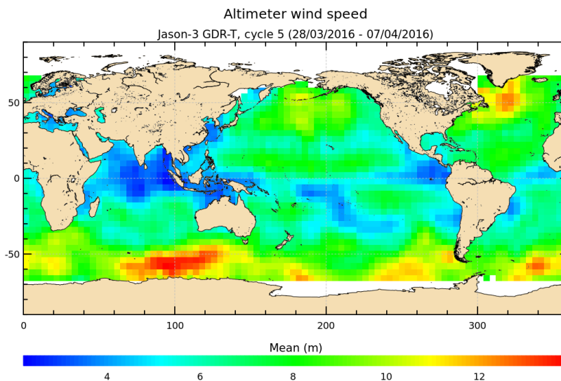
FIGURE 10 – Altimeter wind speed for cycle 005.
