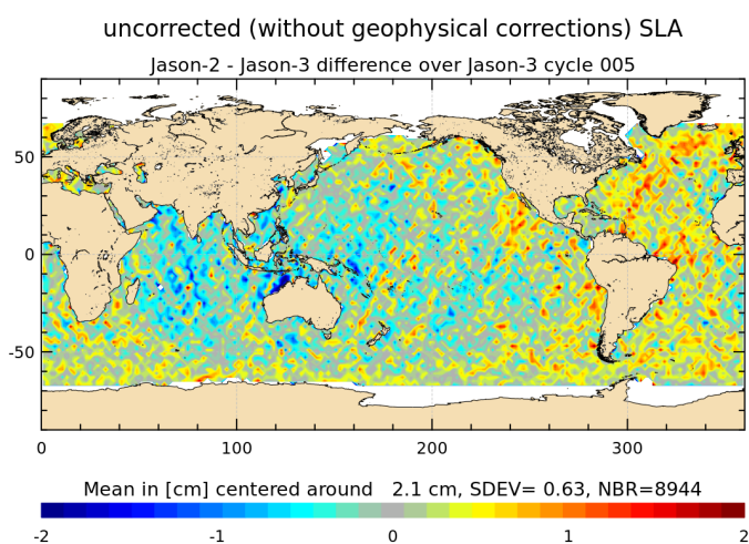
FIGURE 19 – Jason-2 – Jason-3 SLA differences (without corrections) for cycle 005.
