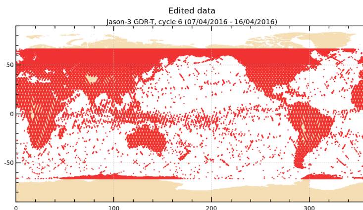
FIGURE 2 – Edited measurements for cycle 006.
