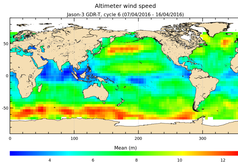
FIGURE 9 – Altimeter wind speed for cycle 006.
