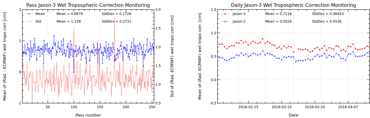
FIGURE 11 – Pass monitoring of wet troposphere differences between radiometer and ECMWF model for Jason-3 cycle 006 (left) and Jason-3 versus Jason-2 daily monitoring of wet troposphere differences between radiometer and ECMWF model (right).
