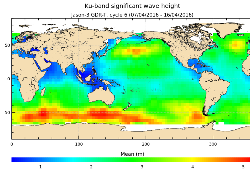
FIGURE 5 – Significant wave height for cycle 006.
