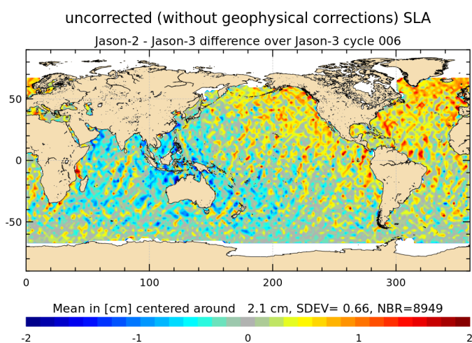
FIGURE 18 – Jason-2 – Jason-3 SLA differences (without corrections) for cycle 006.
