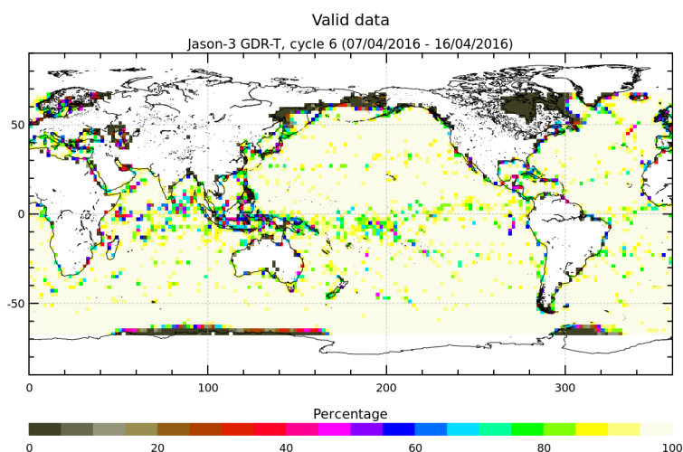
FIGURE 3 – Percentage of valid measurements for cycle 006.
