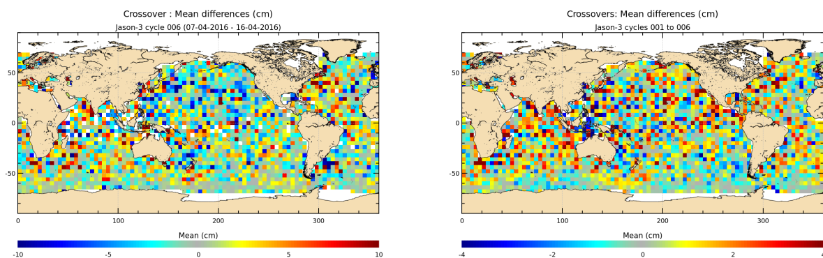
FIGURE 12 – Mean SSH at crossovers for cycle 006 (left) and over the whole Jason-3 period (right).
