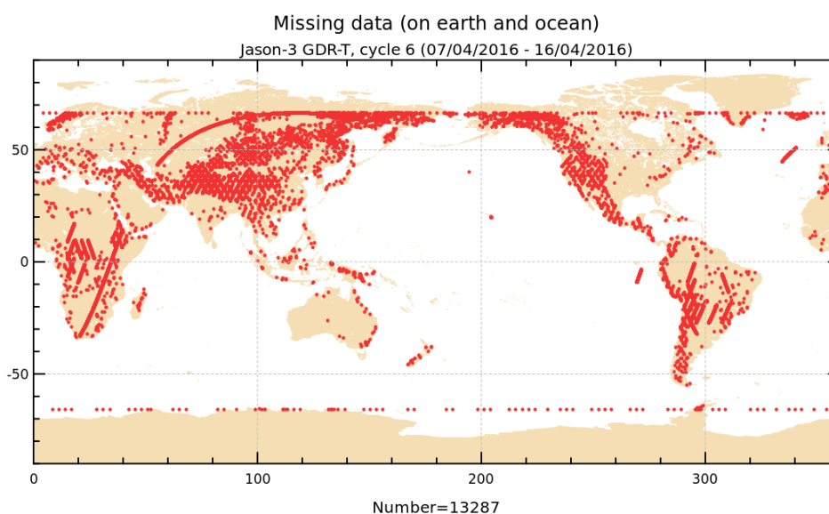
FIGURE 1 – Missing measurements for cycle 006.
