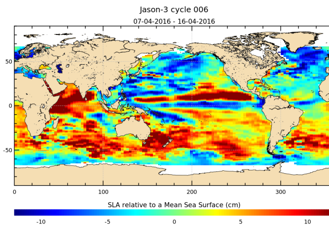
FIGURE 17 – Sea level anomaly relative to MSS for cycle 006.
