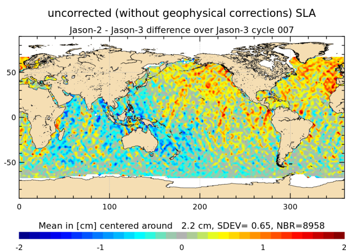
FIGURE 19 – Jason-2 – Jason-3 SLA differences (without corrections) for cycle 007.
