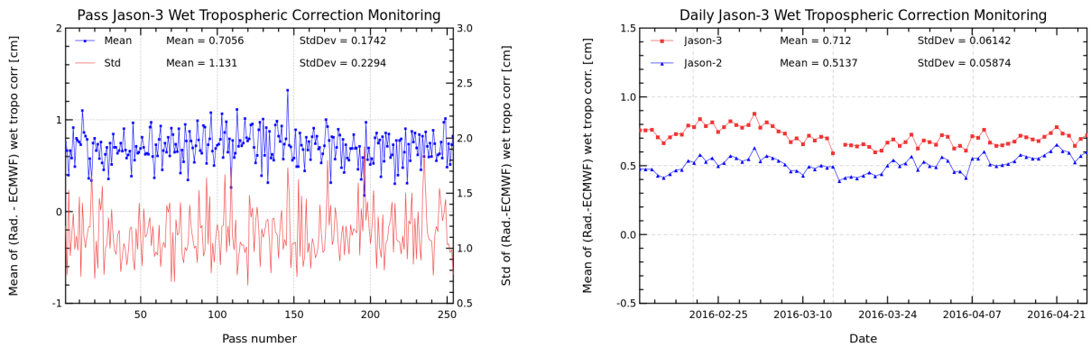
FIGURE 12 – Pass monitoring of wet troposphere differences between radiometer and ECMWF model for Jason-3 cycle 007 (left) and Jason-3 versus Jason-2 daily monitoring of wet troposphere differences between radiometer and ECMWF model (right).
