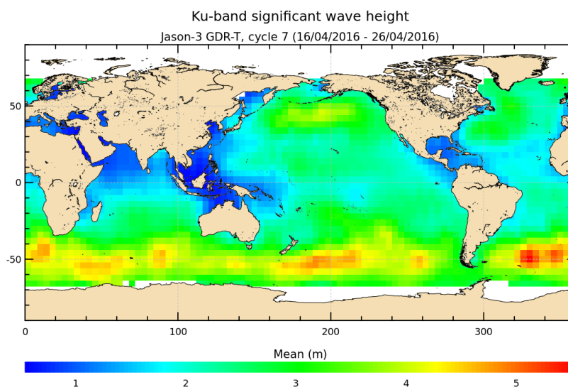
FIGURE 6 – Significant wave height for cycle 007.
