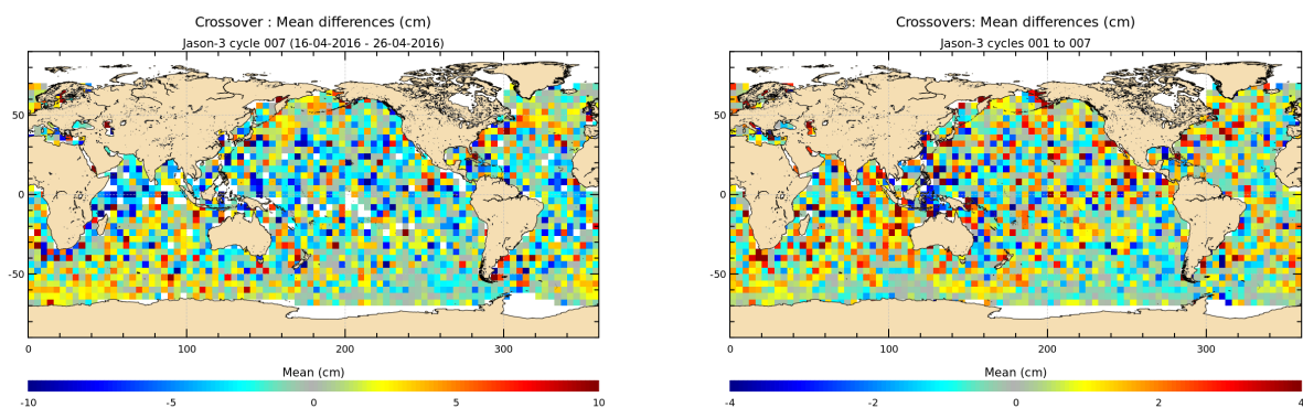
FIGURE 13 – Mean SSH at crossovers for cycle 007 (left) and over the whole Jason-3 period (right).
