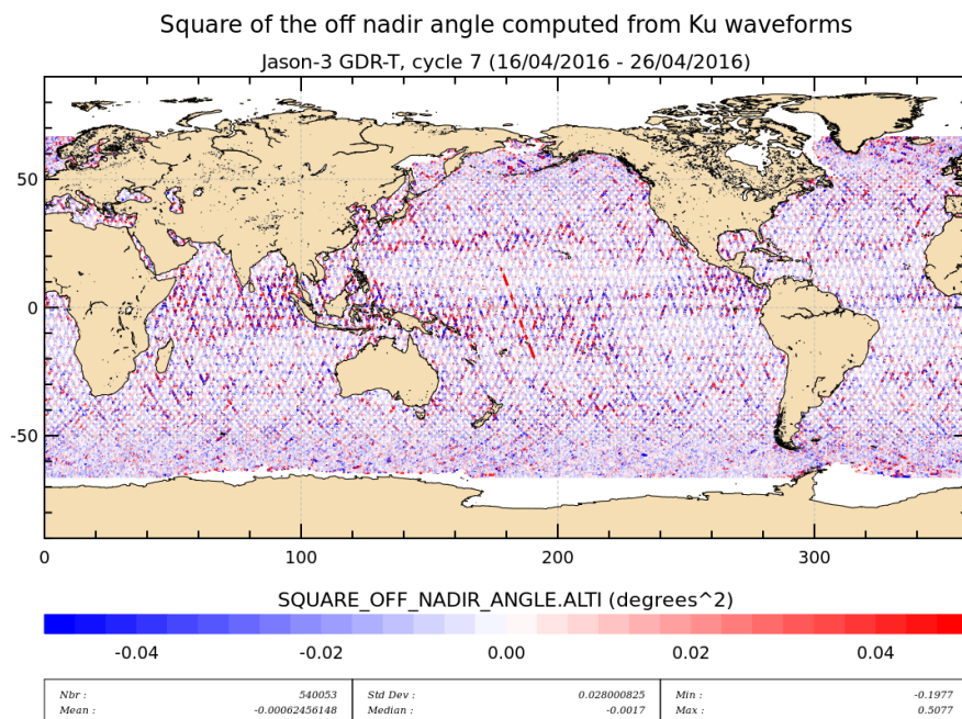
FIGURE 4 – Apparent squared mispointing from waveforms for cycle 007.
