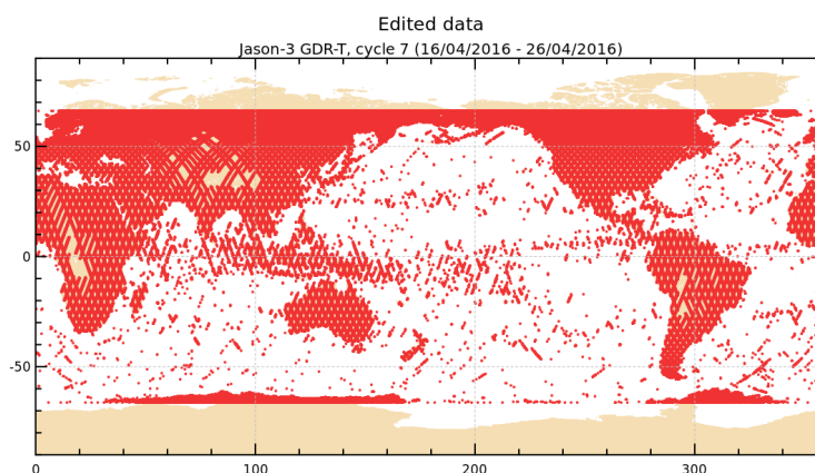
FIGURE 2 – Edited measurements for cycle 007.
