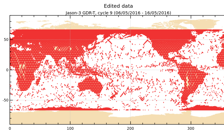
FIGURE 2 – Edited measurements for cycle 009.
