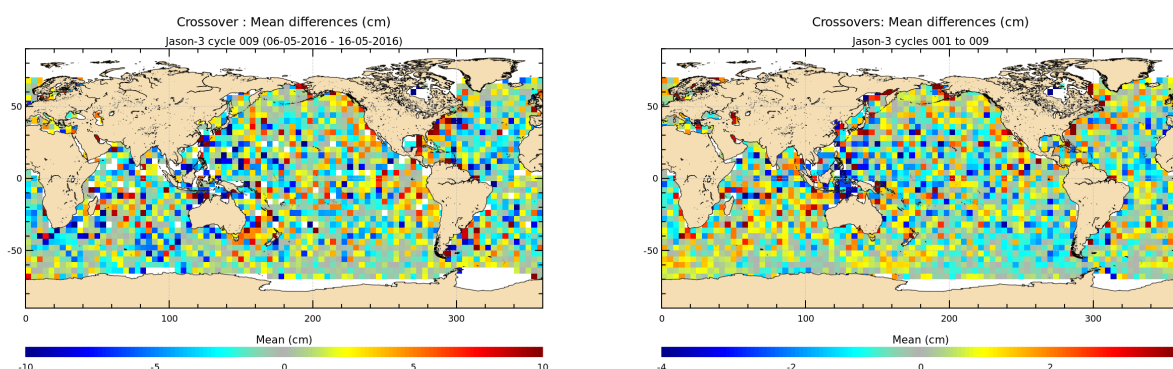
FIGURE 12 – Mean SSH at crossovers for cycle 009 (left) and over the whole Jason-3 period (right).
