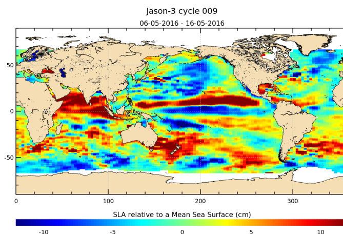
FIGURE 17 – Sea level anomaly relative to MSS for cycle 009.
