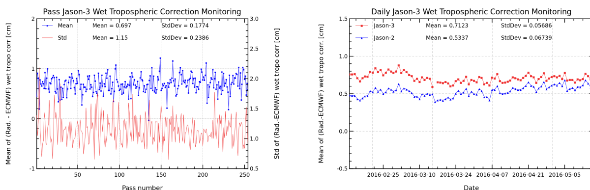
FIGURE 11 – Pass monitoring of wet troposphere differences between radiometer and ECMWF model for Jason-3 cycle 009 (left) and Jason-3 versus Jason-2 daily monitoring of wet troposphere differences between radiometer and ECMWF model (right).
