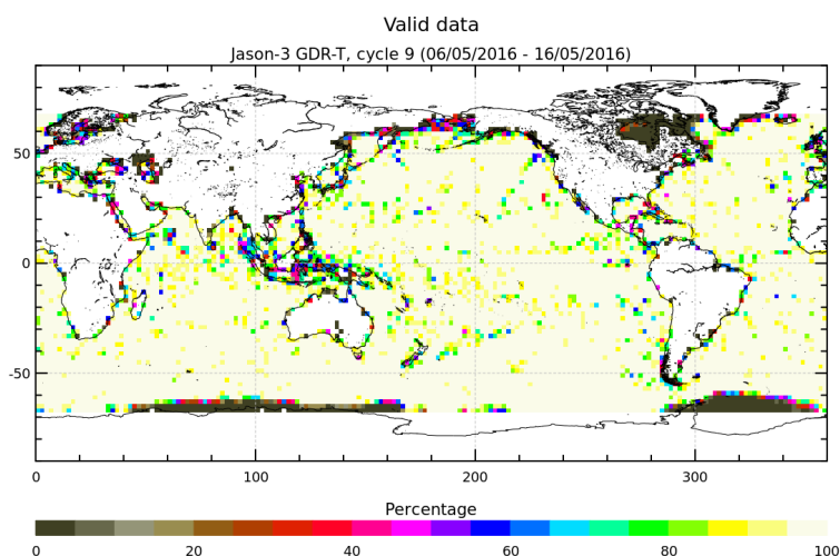
FIGURE 3 – Percentage of valid measurements for cycle 009.
