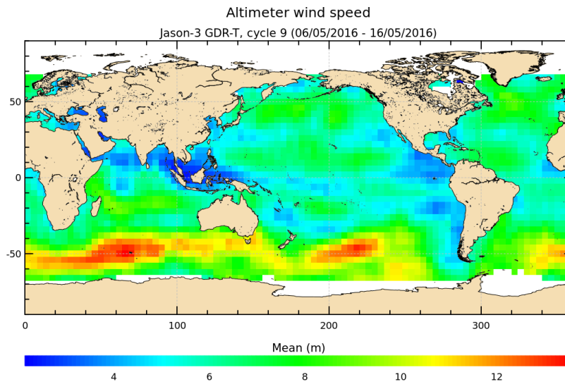
FIGURE 9 – Altimeter wind speed for cycle 009.
