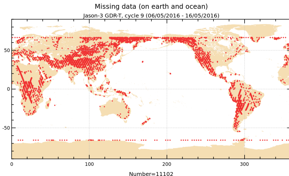
FIGURE 1 – Missing measurements for cycle 009.
