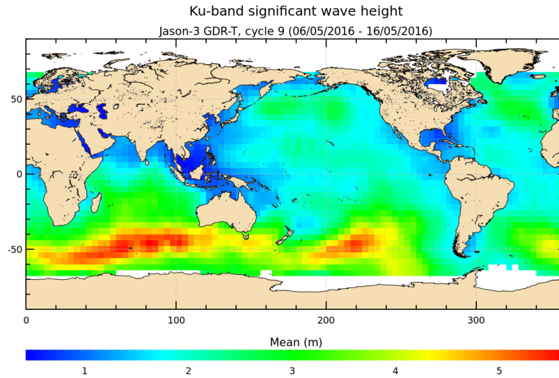
FIGURE 5 – Significant wave height for cycle 009.
