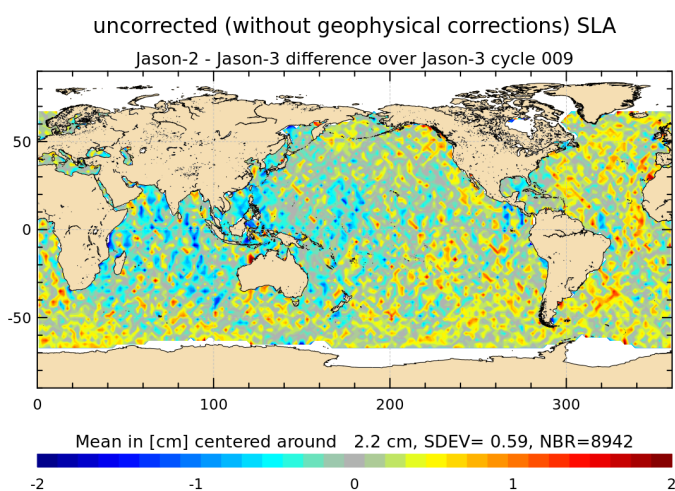
FIGURE 18 – Jason-2 – Jason-3 SLA differences (without corrections) for cycle 009.
