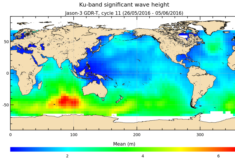
FIGURE 5 – Significant wave height for cycle 011.
