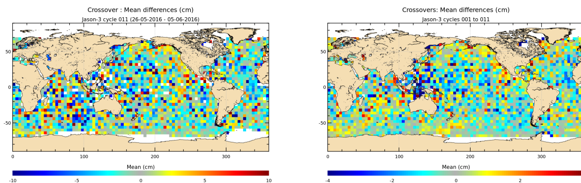
FIGURE 12 – Mean SSH at crossovers for cycle 011 (left) and over the whole Jason-3 period (right).
