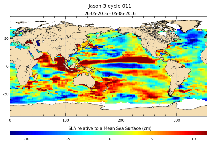
FIGURE 17 – Sea level anomaly relative to MSS for cycle 011.
