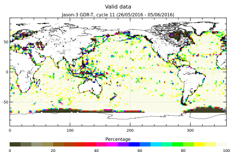
FIGURE 3 – Percentage of valid measurements for cycle 011.
