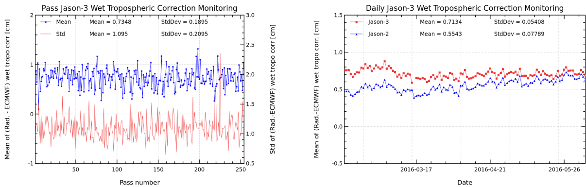
FIGURE 11 – Pass monitoring of wet troposphere differences between radiometer and ECMWF model for Jason-3 cycle 011 (left) and Jason-3 versus Jason-2 daily monitoring of wet troposphere differences between radiometer and ECMWF model (right).
