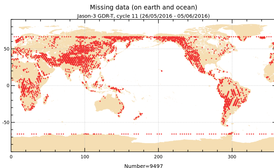
FIGURE 1 – Missing measurements for cycle 011.
