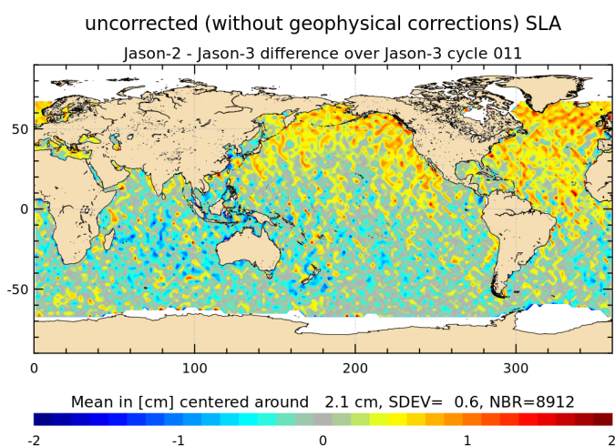
FIGURE 18 – Jason-2 – Jason-3 SLA differences (without corrections) for cycle 011.
