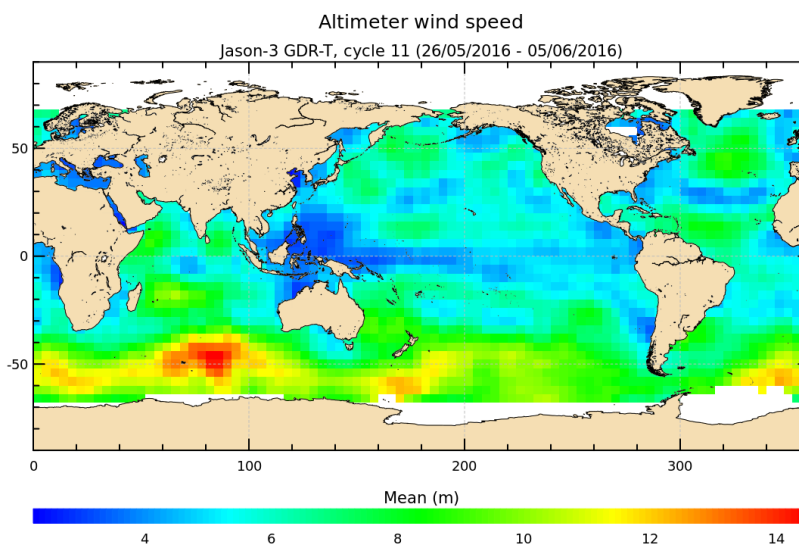
FIGURE 9 – Altimeter wind speed for cycle 011.
