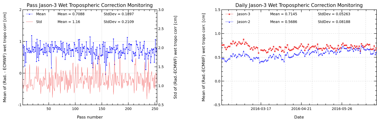
FIGURE 11 – Pass monitoring of wet troposphere differences between radiometer and ECMWF model for Jason-3 cycle 013 (left) and Jason-3 versus Jason-2 daily monitoring of wet troposphere differences between radiometer and ECMWF model (right).
