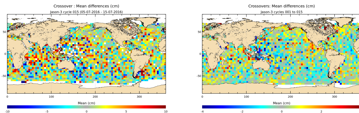
FIGURE 13 – Mean SSH at crossovers for cycle 015 (left) and over the whole Jason-3 period (right).
