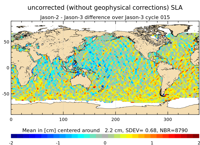
FIGURE 19 – Jason-2 – Jason-3 SLA differences (without corrections) for cycle 015.
