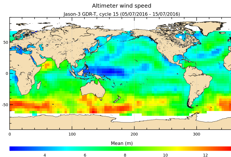
FIGURE 10 – Altimeter wind speed for cycle 015.
