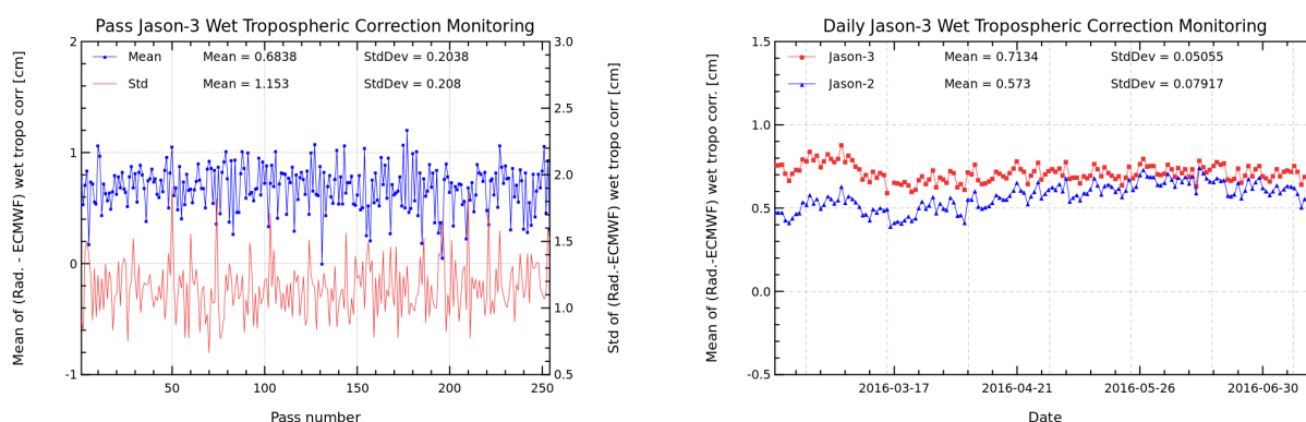
FIGURE 12 – Pass monitoring of wet troposphere differences between radiometer and ECMWF model for Jason-3 cycle 015 (left) and Jason-3 versus Jason-2 daily monitoring of wet troposphere differences between radiometer and ECMWF model (right).
