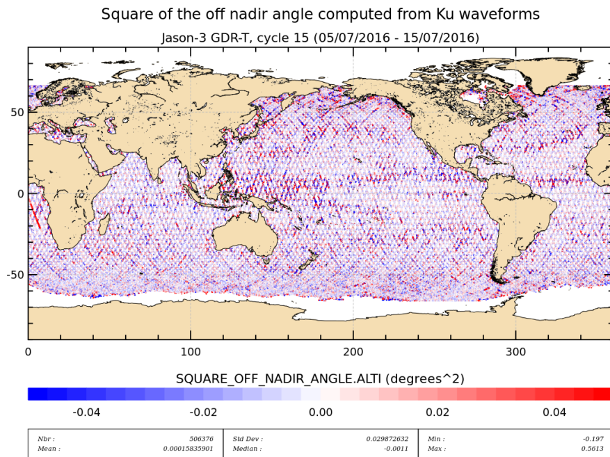
FIGURE 4 – Apparent squared mispointing from waveforms for cycle 015.
