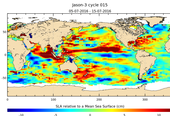
FIGURE 18 – Sea level anomaly relative to MSS for cycle 015.
