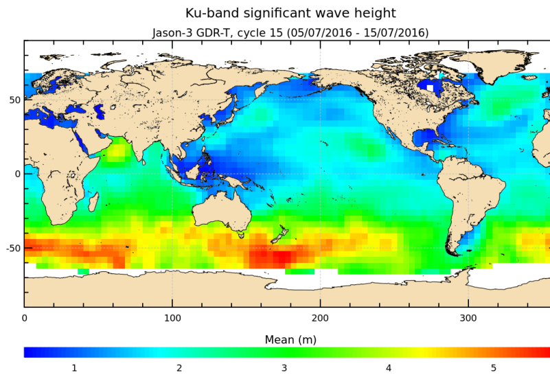
FIGURE 6 – Significant wave height for cycle 015.
