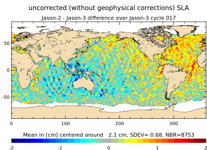
FIGURE 18 – Jason-2 – Jason-3 SLA differences (without corrections) for cycle 017.
