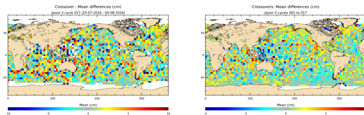
FIGURE 12 – Mean SSH at crossovers for cycle 017 (left) and over the whole Jason-3 period (right).
