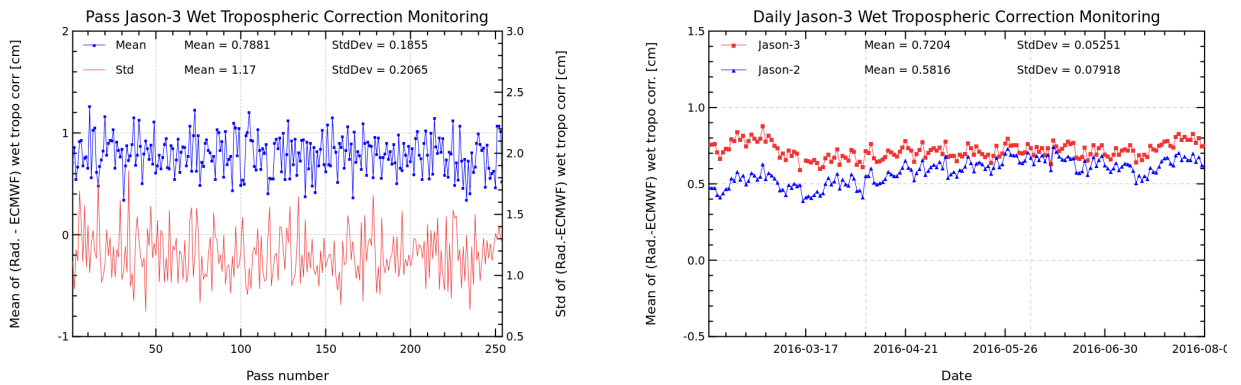
FIGURE 11 – Pass monitoring of wet troposphere differences between radiometer and ECMWF model for Jason-3 cycle 017 (left) and Jason-3 versus Jason-2 daily monitoring of wet troposphere differences between radiometer and ECMWF model (right).
