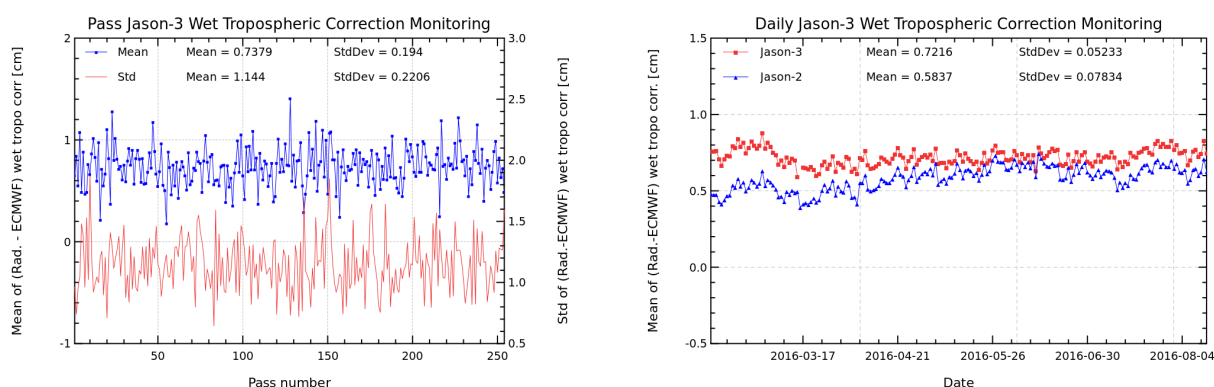
FIGURE 11 – Pass monitoring of wet troposphere differences between radiometer and ECMWF model for Jason-3 cycle 018 (left) and Jason-3 versus Jason-2 daily monitoring of wet troposphere differences between radiometer and ECMWF model (right).
