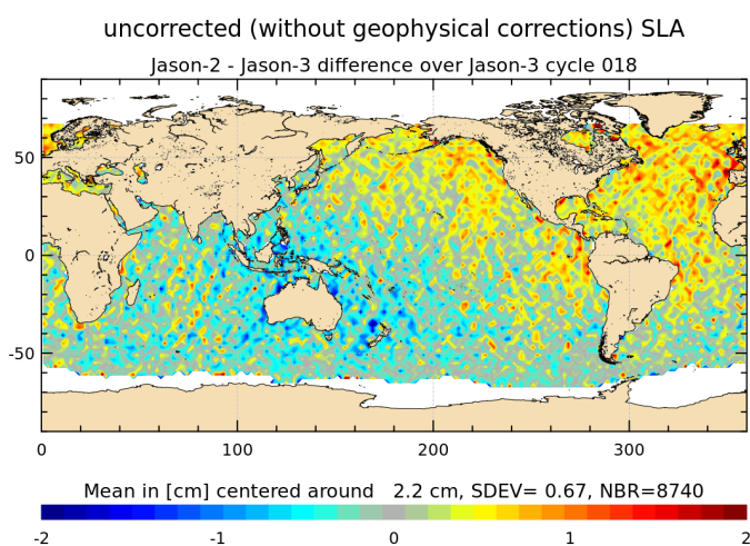
FIGURE 18 – Jason-2 – Jason-3 SLA differences (without corrections) for cycle 018.
