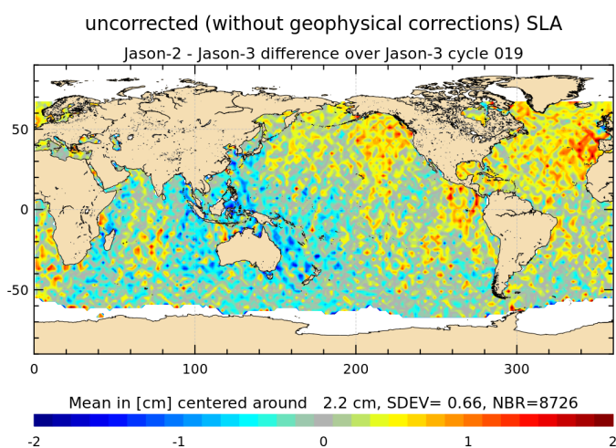
FIGURE 18 – Jason-2 – Jason-3 SLA differences (without corrections) for cycle 019.
