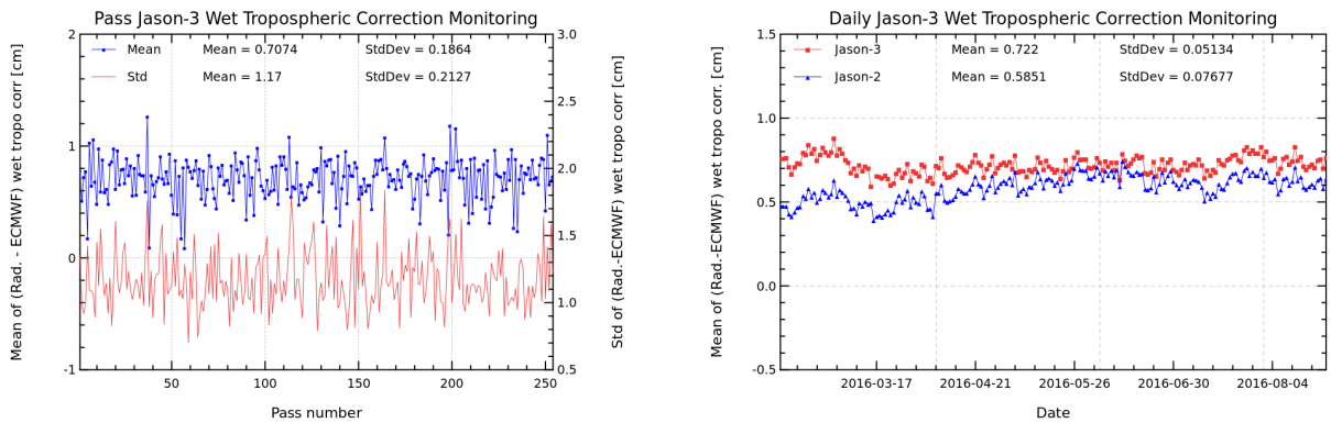
FIGURE 11 – Pass monitoring of wet troposphere differences between radiometer and ECMWF model for Jason-3 cycle 019 (left) and Jason-3 versus Jason-2 daily monitoring of wet troposphere differences between radiometer and ECMWF model (right).
