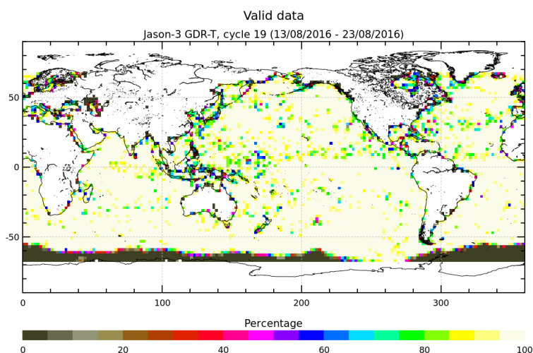
FIGURE 3 – Percentage of valid measurements for cycle 019.
