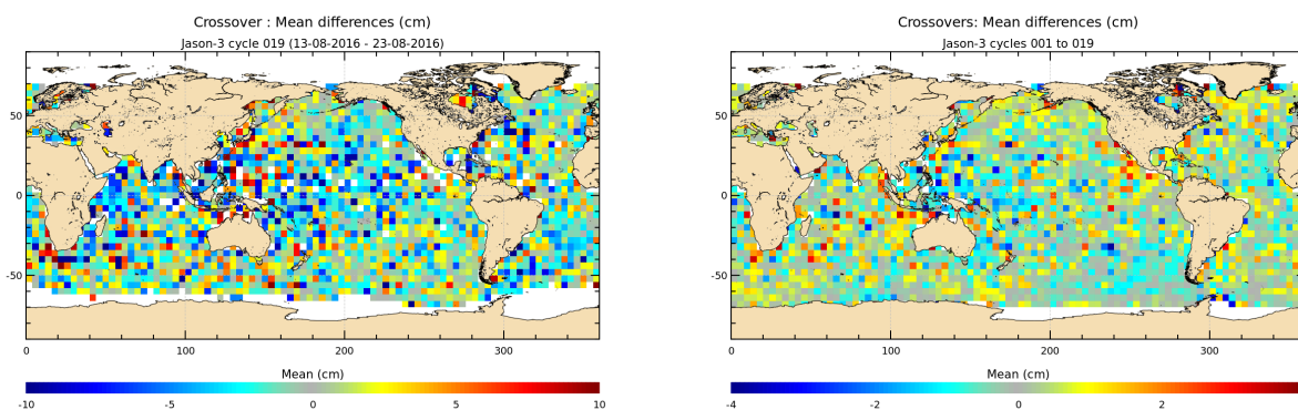
FIGURE 12 – Mean SSH at crossovers for cycle 019 (left) and over the whole Jason-3 period (right).
