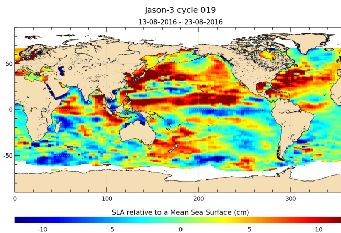
FIGURE 17 – Sea level anomaly relative to MSS for cycle 019.
