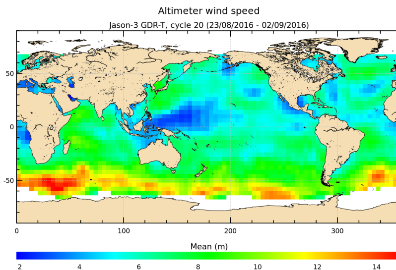
FIGURE 9 – Altimeter wind speed for cycle 020.
