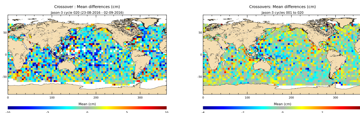
FIGURE 12 – Mean SSH at crossovers for cycle 020 (left) and over the whole Jason-3 period (right).
