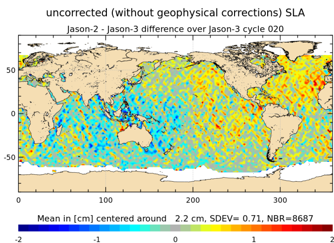
FIGURE 18 – Jason-2 – Jason-3 SLA differences (without corrections) for cycle 020.
