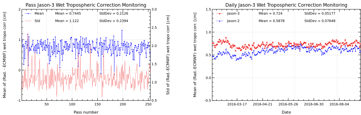
FIGURE 11 – Pass monitoring of wet troposphere differences between radiometer and ECMWF model for Jason-3 cycle 020 (left) and Jason-3 versus Jason-2 daily monitoring of wet troposphere differences between radiometer and ECMWF model (right).
