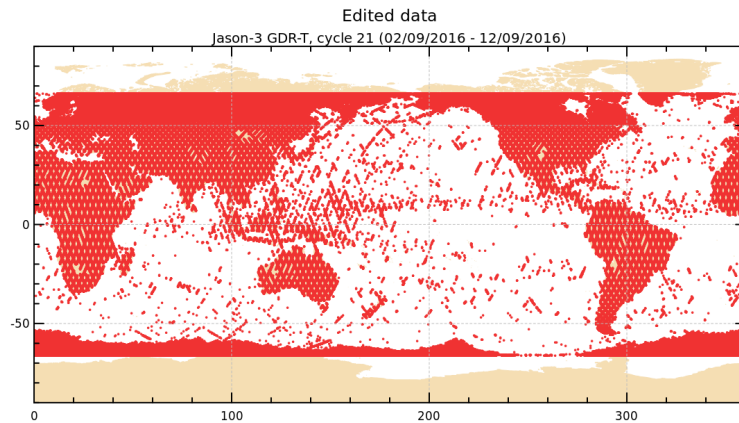
FIGURE 2 – Edited measurements for cycle 021.
