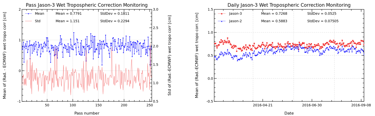
FIGURE 11 – Pass monitoring of wet troposphere differences between radiometer and ECMWF model for Jason-3 cycle 021 (left) and Jason-3 versus Jason-2 daily monitoring of wet troposphere differences between radiometer and ECMWF model (right).
