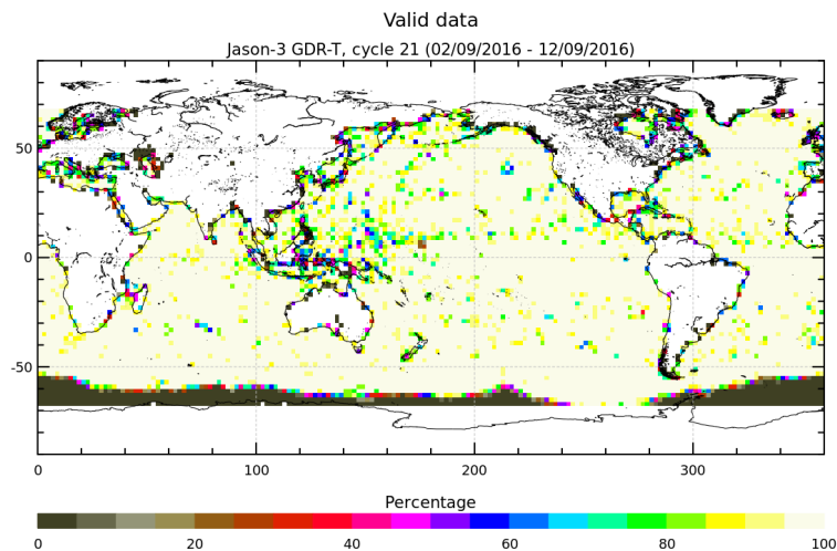
FIGURE 3 – Percentage of valid measurements for cycle 021.
