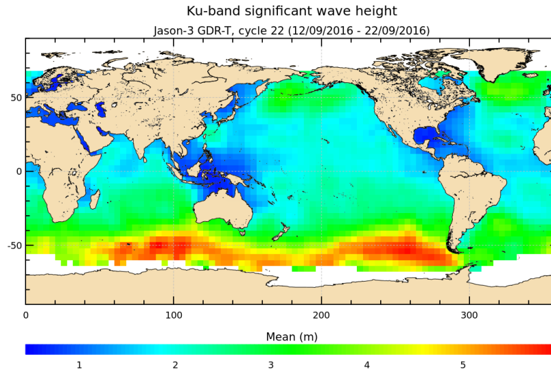
FIGURE 5 – Significant wave height for cycle 022.
