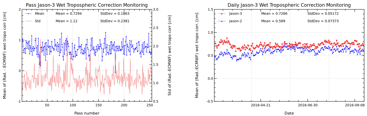
FIGURE 11 – Pass monitoring of wet troposphere differences between radiometer and ECMWF model for Jason-3 cycle 022 (left) and Jason-3 versus Jason-2 daily monitoring of wet troposphere differences between radiometer and ECMWF model (right).
