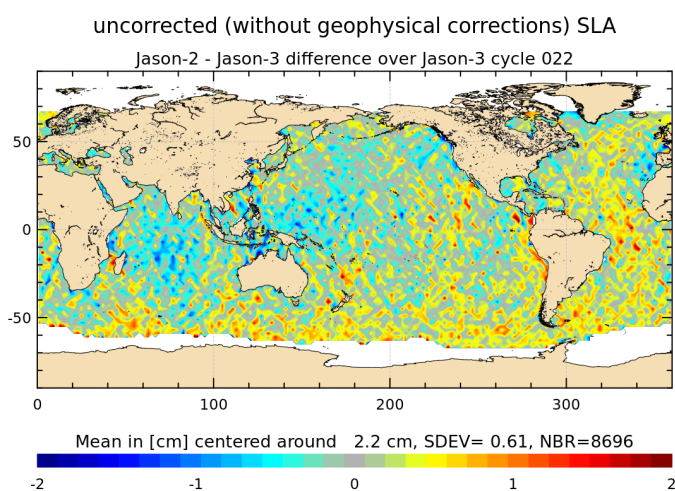
FIGURE 18 – Jason-2 – Jason-3 SLA differences (without corrections) for cycle 022.
