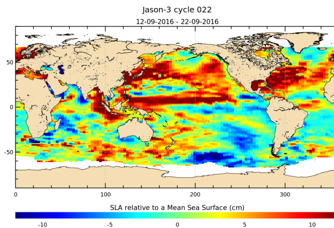
FIGURE 17 – Sea level anomaly relative to MSS for cycle 022.
