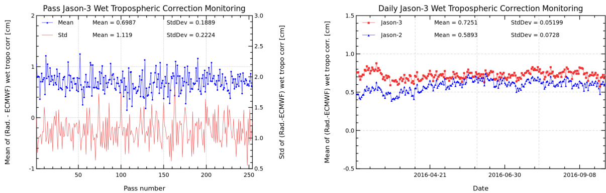
FIGURE 11 – Pass monitoring of wet troposphere differences between radiometer and ECMWF model for Jason-3 cycle 023 (left) and Jason-3 versus Jason-2 daily monitoring of wet troposphere differences between radiometer and ECMWF model (right).
