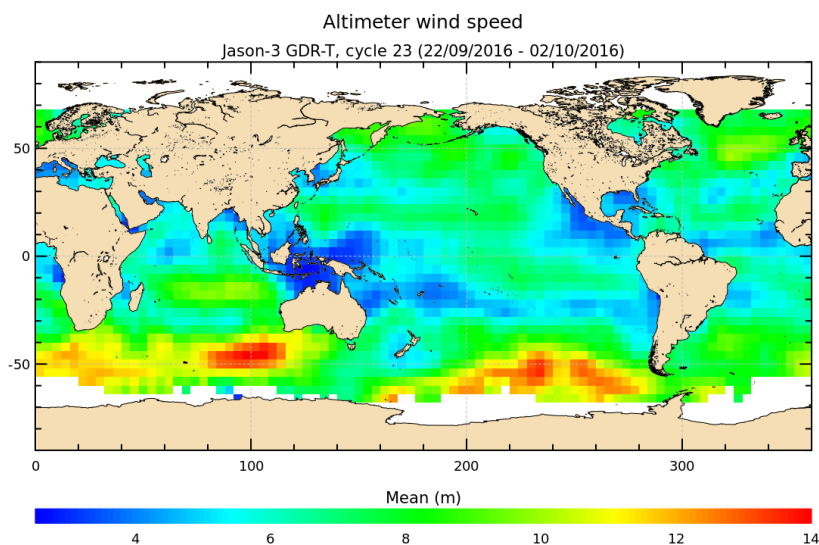
FIGURE 9 – Altimeter wind speed for cycle 023.
