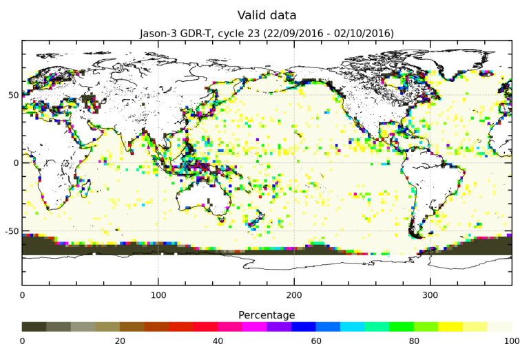
FIGURE 3 – Percentage of valid measurements for cycle 023.
