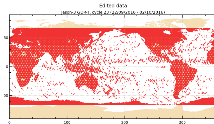
FIGURE 2 – Edited measurements for cycle 023.
