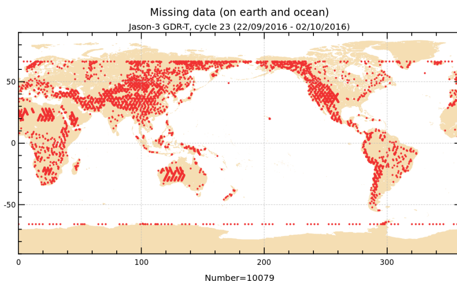
FIGURE 1 – Missing measurements for cycle 023.
