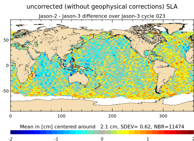
FIGURE 18 – Jason-2 – Jason-3 SLA differences (without corrections) for cycle 023.
