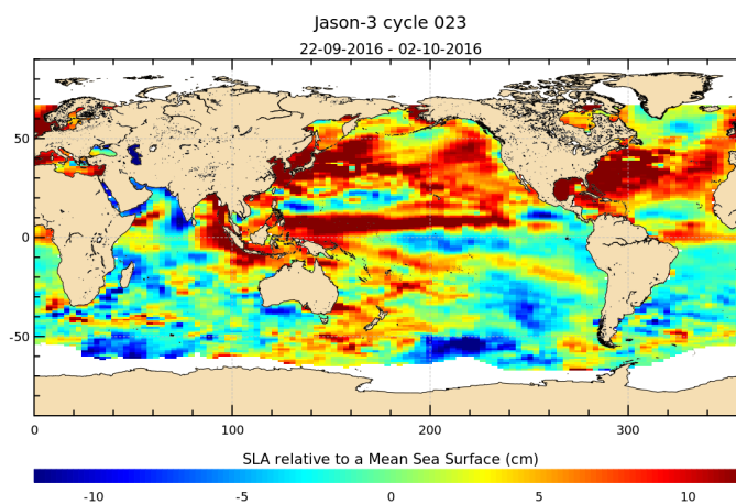
FIGURE 17 – Sea level anomaly relative to MSS for cycle 023.
