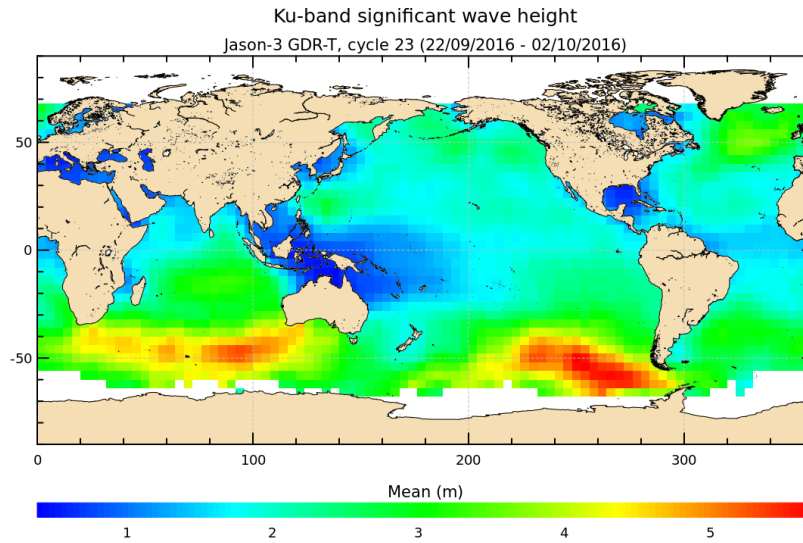
FIGURE 5 – Significant wave height for cycle 023.
