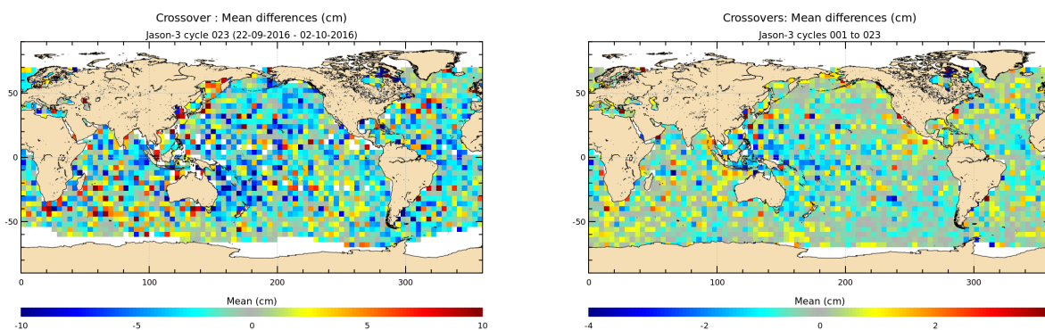
FIGURE 12 – Mean SSH at crossovers for cycle 023 (left) and over the whole Jason-3 period (right).
