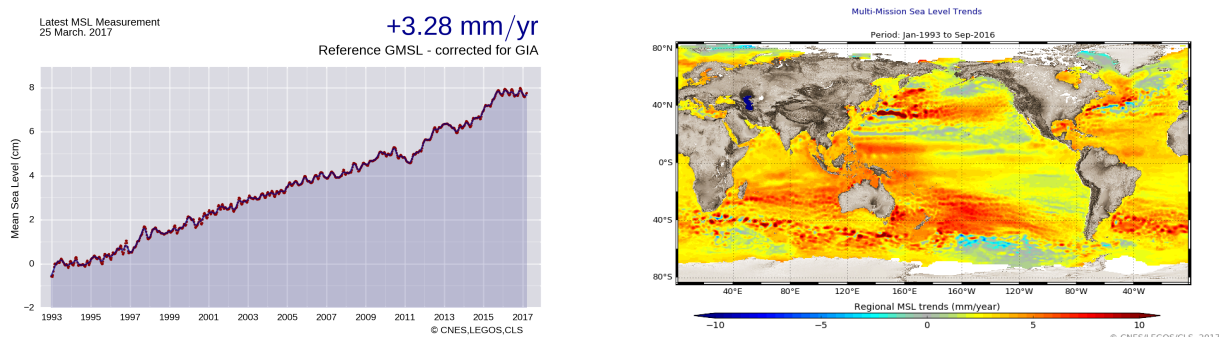
FIGURE 19 – Global (left) and regional (right) MSL trends from 1993 onwards.
