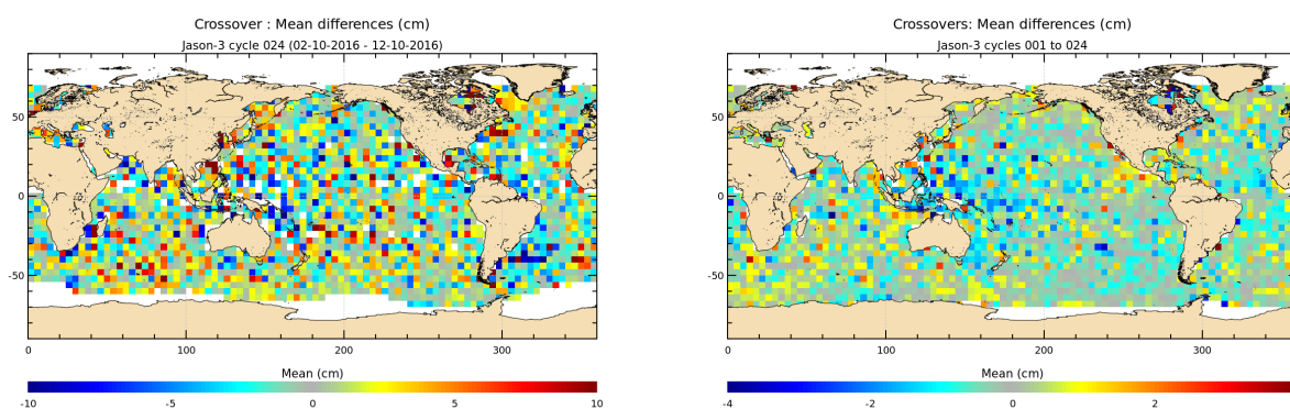
FIGURE 12 – Mean SSH at crossovers for cycle 024 (left) and over the whole Jason-3 period (right).
