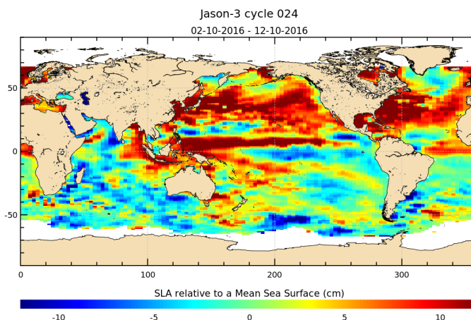
FIGURE 17 – Sea level anomaly relative to MSS for cycle 024.
