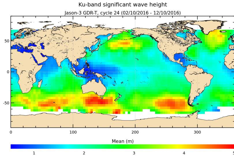
FIGURE 5 – Significant wave height for cycle 024.
