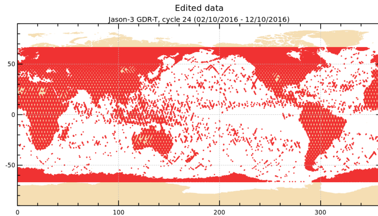
FIGURE 2 – Edited measurements for cycle 024.
