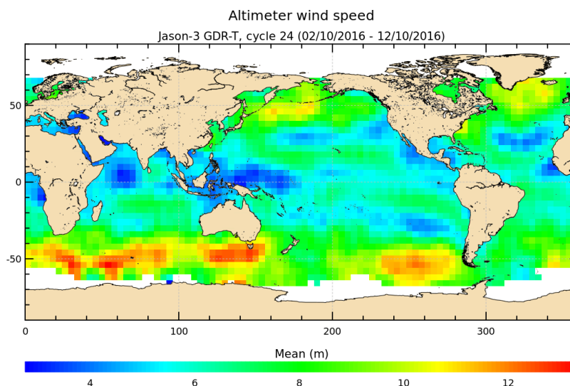
FIGURE 9 – Altimeter wind speed for cycle 024.
