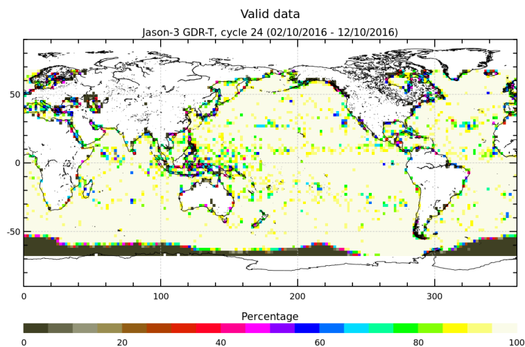
FIGURE 3 – Percentage of valid measurements for cycle 024.
