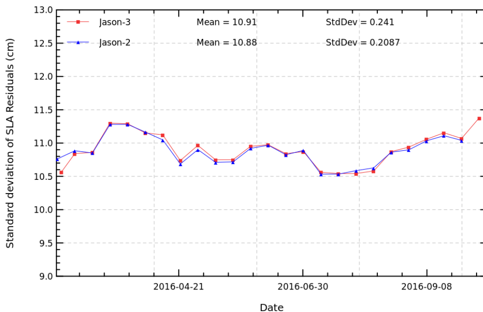
FIGURE 18 – Cyclic monitoring standard deviation of along track SLA for Jason-3 and Jason-2.
