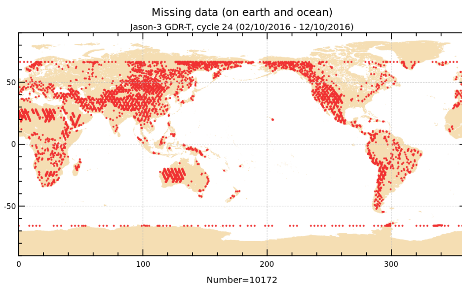
FIGURE 1 – Missing measurements for cycle 024.
