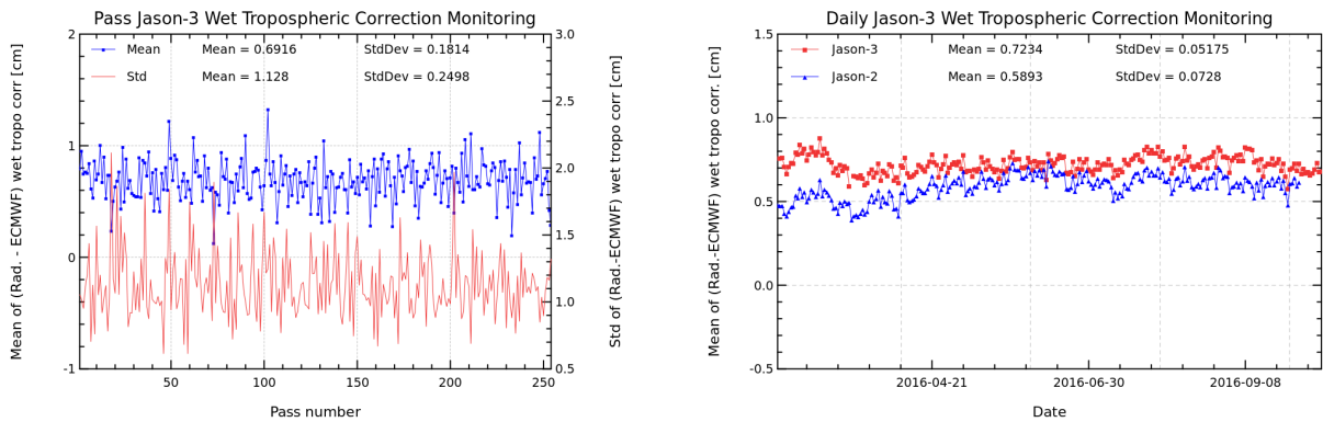
FIGURE 11 – Pass monitoring of wet troposphere differences between radiometer and ECMWF model for Jason-3 cycle 024 (left) and Jason-3 versus Jason-2 daily monitoring of wet troposphere differences between radiometer and ECMWF model (right).
