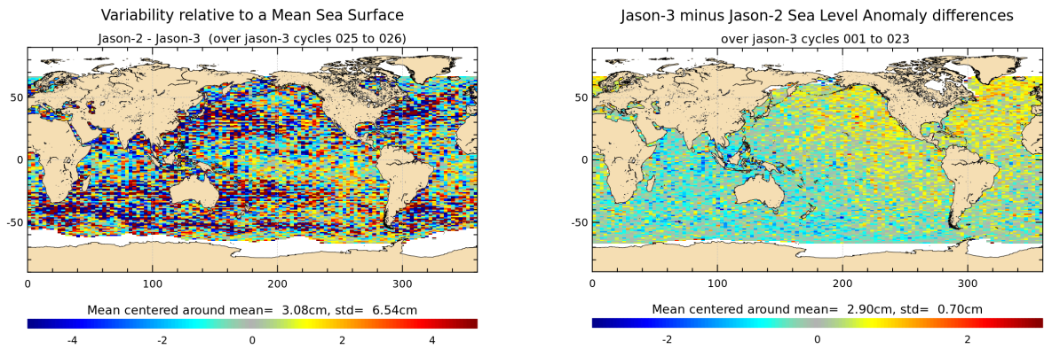
FIGURE 18 – Jason-2 – Jason-3 SLA differences averaged over Jason-3 period from cycle 025 until cycle 026 (left), and for tandem phase (cycle 001 to 023) (right).
