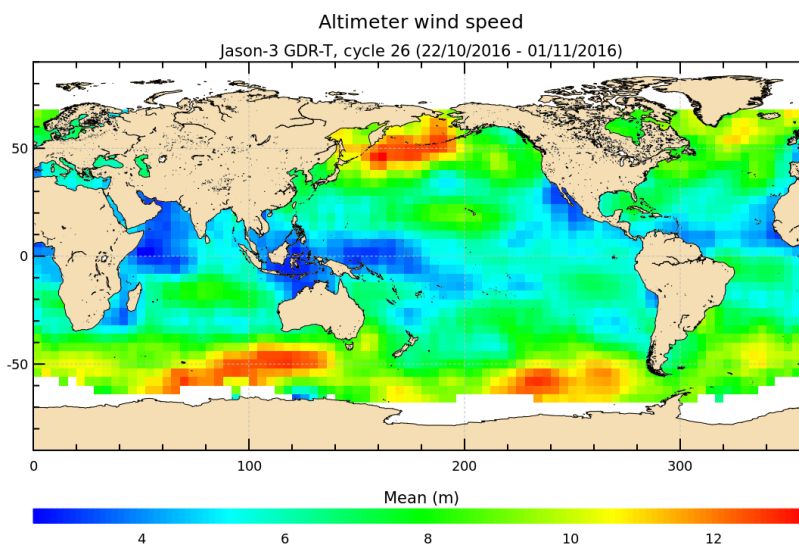
FIGURE 9 – Altimeter wind speed for cycle 026.
