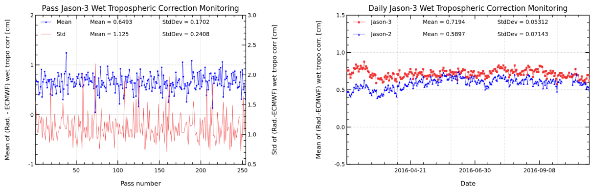
FIGURE 11 – Pass monitoring of wet troposphere differences between radiometer and ECMWF model for Jason-3 cycle 026 (left) and Jason-3 versus Jason-2 daily monitoring of wet troposphere differences between radiometer and ECMWF model (right).
