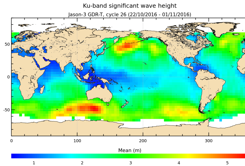
FIGURE 5 – Significant wave height for cycle 026.
