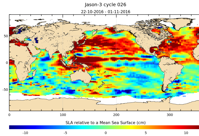
FIGURE 17 – Sea level anomaly relative to MSS for cycle 026.
