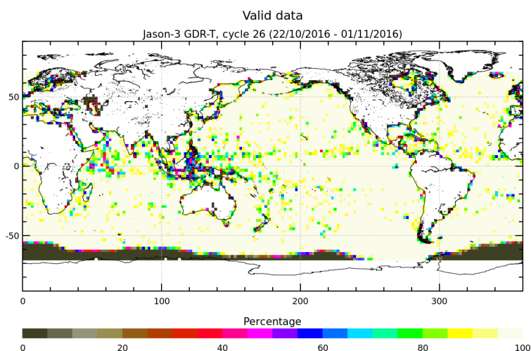
FIGURE 3 – Percentage of valid measurements for cycle 026.
