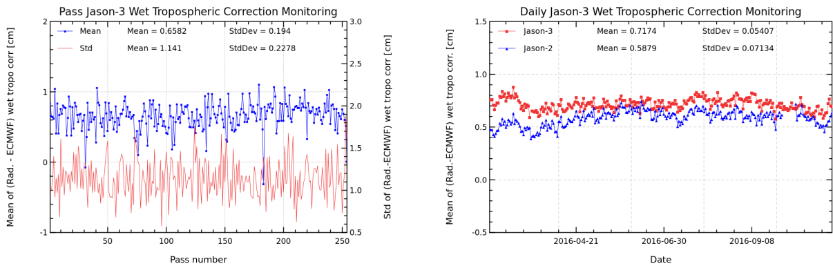
FIGURE 11 – Pass monitoring of wet troposphere differences between radiometer and ECMWF model for Jason-3 cycle 027 (left) and Jason-3 versus Jason-2 daily monitoring of wet troposphere differences between radiometer and ECMWF model (right).
