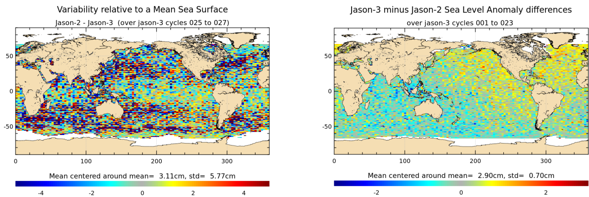
FIGURE 18 – Jason-2 – Jason-3 SLA differences averaged over Jason-3 period from cycle 025 until cycle 027 (left), and for tandem phase (cycle 001 to 023) (right).
