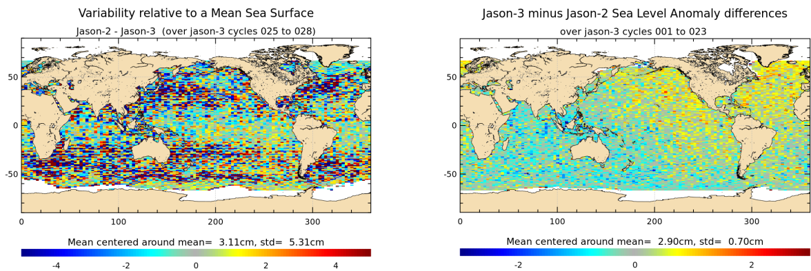
FIGURE 18 – Jason-2 – Jason-3 SLA differences averaged over Jason-3 period from cycle 025 until cycle 028 (left), and for tandem phase (cycle 001 to 023) (right).
