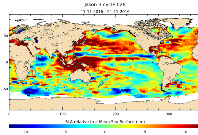
FIGURE 17 – Sea level anomaly relative to MSS for cycle 028.
