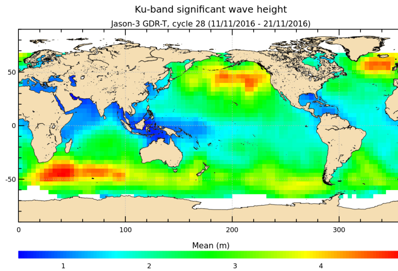
FIGURE 5 – Significant wave height for cycle 028.
