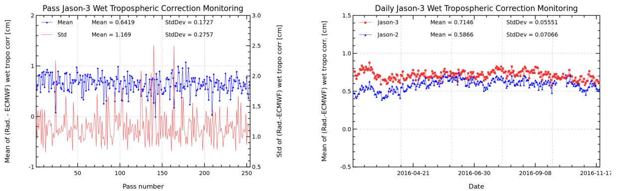
FIGURE 11 – Pass monitoring of wet troposphere differences between radiometer and ECMWF model for Jason-3 cycle 028 (left) and Jason-3 versus Jason-2 daily monitoring of wet troposphere differences between radiometer and ECMWF model (right).
