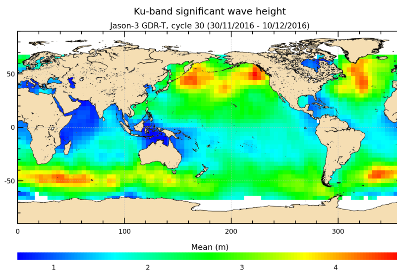
FIGURE 5 – Significant wave height for cycle 030.
