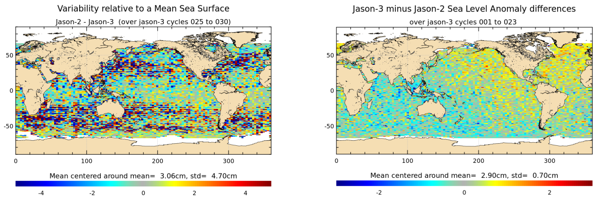
FIGURE 18 – Jason-2 – Jason-3 SLA differences averaged over Jason-3 period from cycle 025 until cycle 030 (left), and for tandem phase (cycle 001 to 023) (right).
