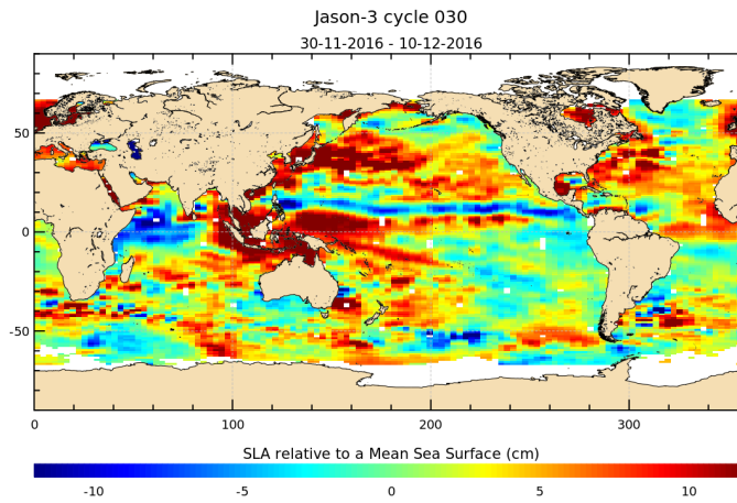
FIGURE 17 – Sea level anomaly relative to MSS for cycle 030.
