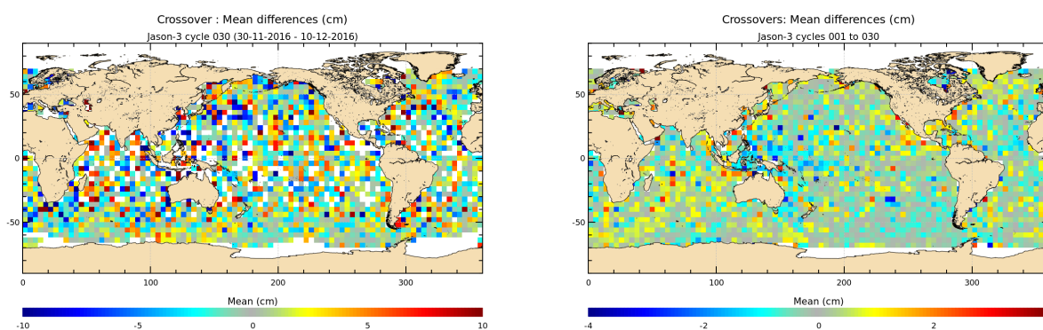
FIGURE 12 – Mean SSH at crossovers for cycle 030 (left) and over the whole Jason-3 period (right).
