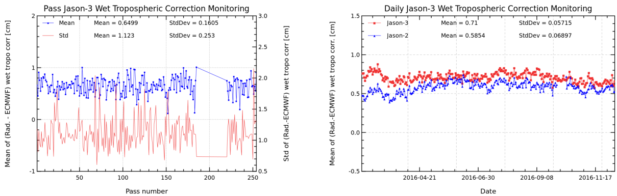
FIGURE 11 – Pass monitoring of wet troposphere differences between radiometer and ECMWF model for Jason-3 cycle 030 (left) and Jason-3 versus Jason-2 daily monitoring of wet troposphere differences between radiometer and ECMWF model (right).
