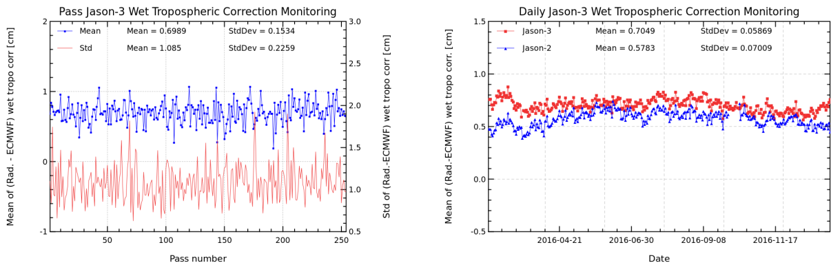
FIGURE 11 – Pass monitoring of wet troposphere differences between radiometer and ECMWF model for Jason-3 cycle 033 (left) and Jason-3 versus Jason-2 daily monitoring of wet troposphere differences between radiometer and ECMWF model (right).
