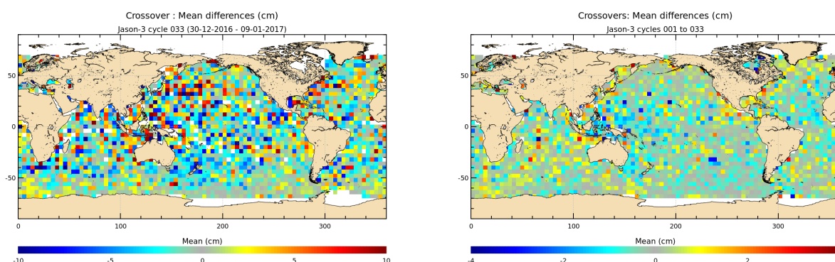
FIGURE 12 – Mean SSH at crossovers for cycle 033 (left) and over the whole Jason-3 period (right).
