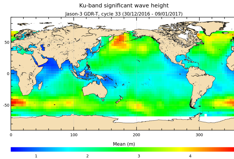
FIGURE 5 – Significant wave height for cycle 033.
