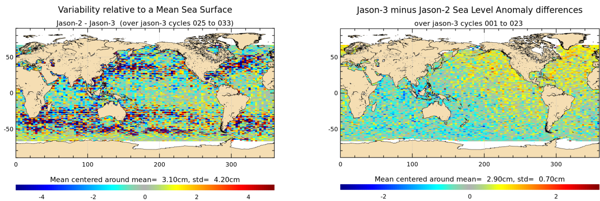
FIGURE 18 – Jason-2 – Jason-3 SLA differences averaged over Jason-3 period from cycle 025 until cycle 033 (left), and for tandem phase (cycle 001 to 023) (right).
