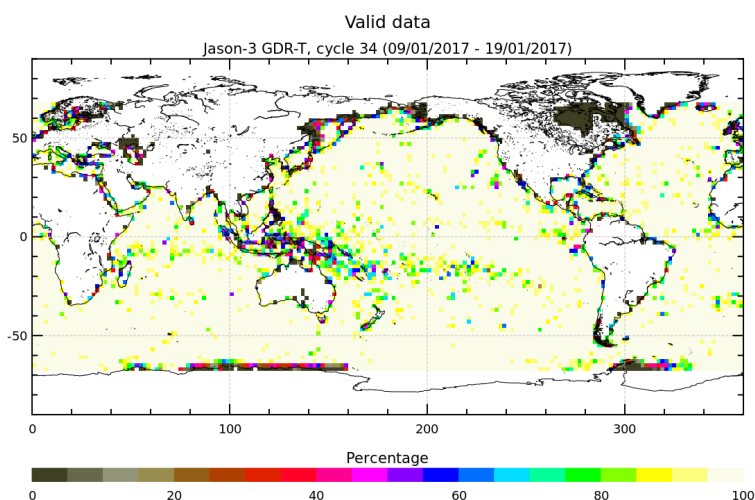
FIGURE 3 – Percentage of valid measurements for cycle 034.
