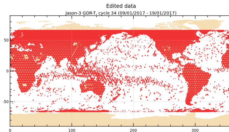
FIGURE 2 – Edited measurements for cycle 034.
