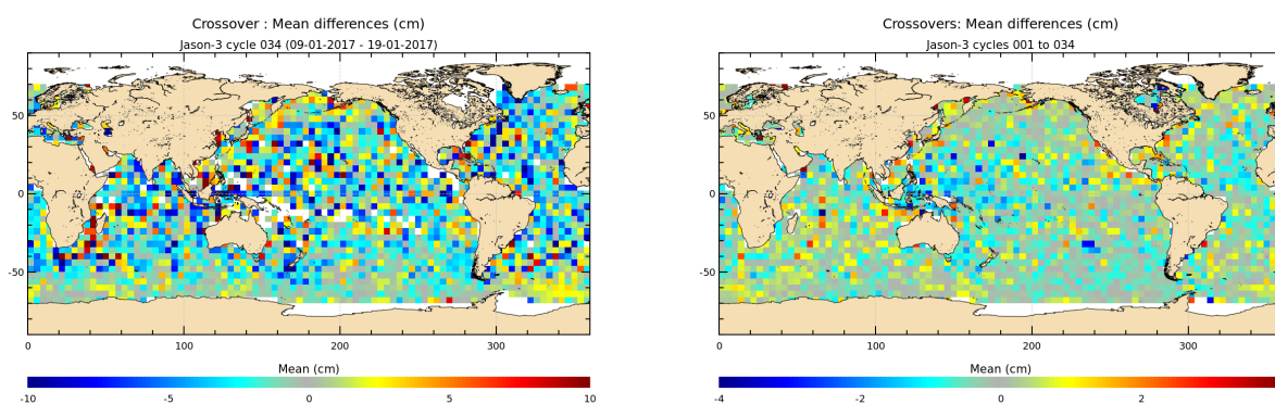
FIGURE 12 – Mean SSH at crossovers for cycle 034 (left) and over the whole Jason-3 period (right).
