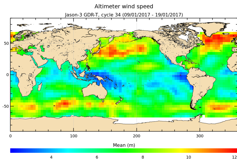
FIGURE 9 – Altimeter wind speed for cycle 034.
