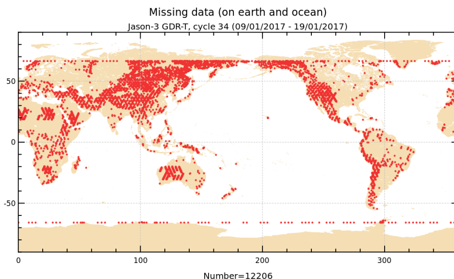
FIGURE 1 – Missing measurements for cycle 034.
