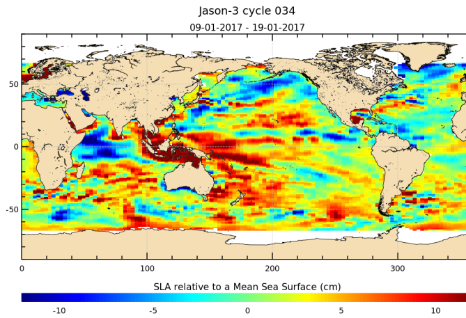
FIGURE 17 – Sea level anomaly relative to MSS for cycle 034.
