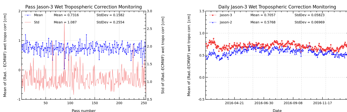
FIGURE 11 – Pass monitoring of wet troposphere differences between radiometer and ECMWF model for Jason-3 cycle 034 (left) and Jason-3 versus Jason-2 daily monitoring of wet troposphere differences between radiometer and ECMWF model (right).
