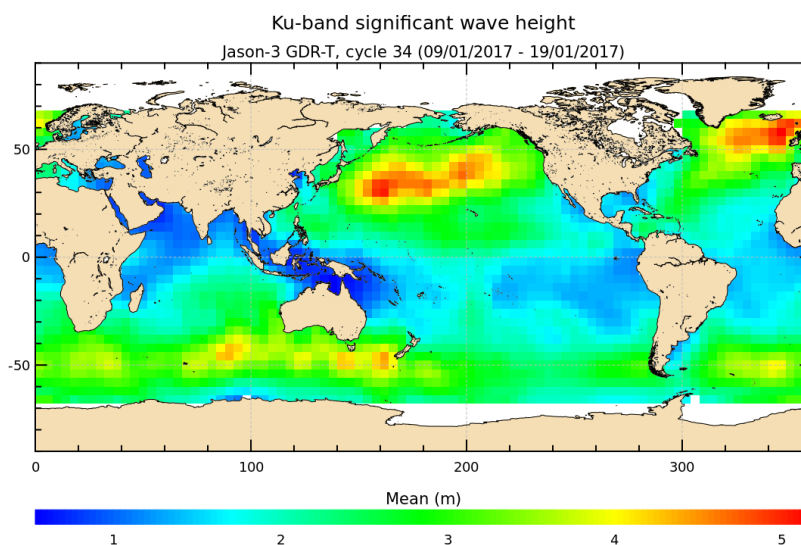
FIGURE 5 – Significant wave height for cycle 034.
