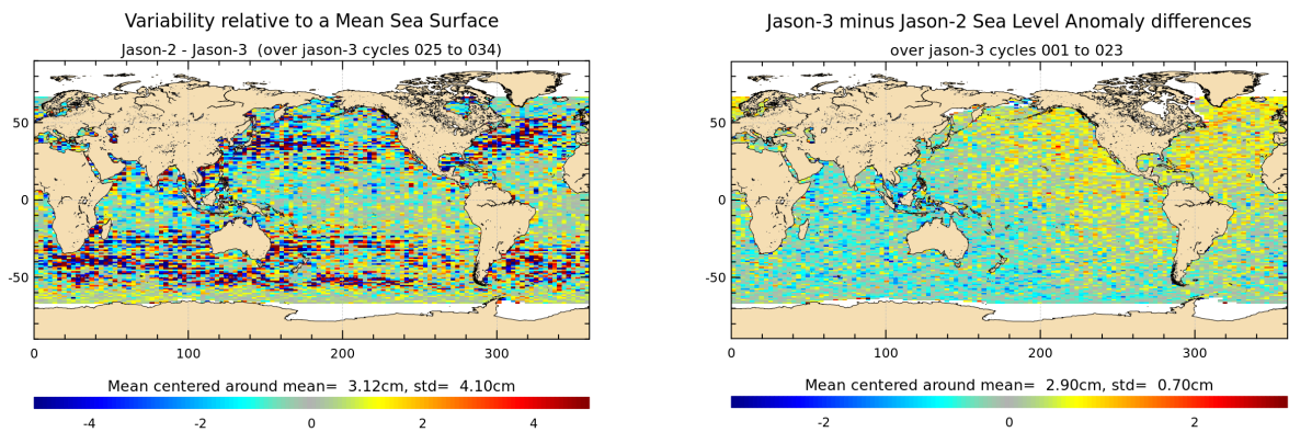
FIGURE 18 – Jason-2 – Jason-3 SLA differences averaged over Jason-3 period from cycle 025 until cycle 034 (left), and for tandem phase (cycle 001 to 023) (right).
