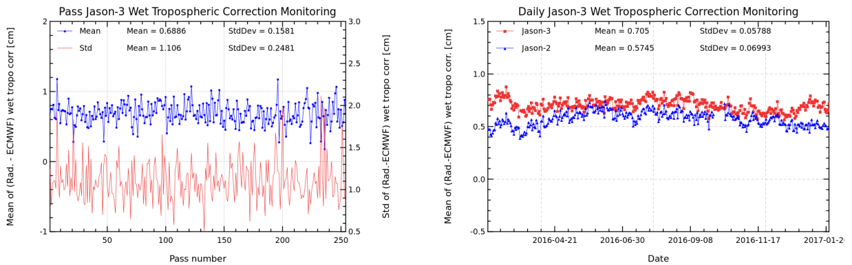
FIGURE 11 – Pass monitoring of wet troposphere differences between radiometer and ECMWF model for Jason-3 cycle 035 (left) and Jason-3 versus Jason-2 daily monitoring of wet troposphere differences between radiometer and ECMWF model (right).
