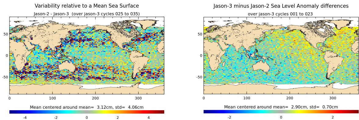
FIGURE 18 – Jason-2 – Jason-3 SLA differences averaged over Jason-3 period from cycle 025 until cycle 035 (left), and for tandem phase (cycle 001 to 023) (right).
