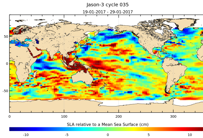
FIGURE 17 – Sea level anomaly relative to MSS for cycle 035.
