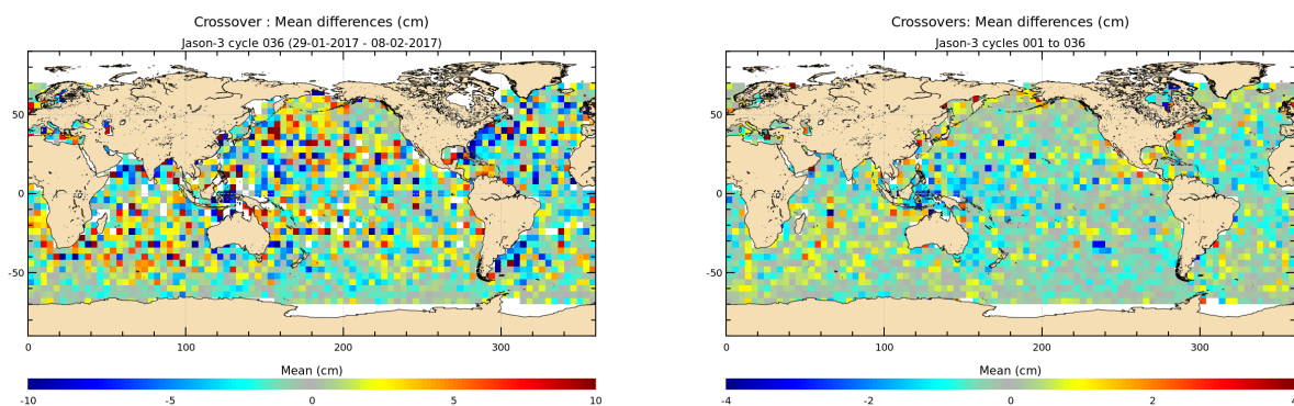
FIGURE 12 – Mean SSH at crossovers for cycle 036 (left) and over the whole Jason-3 period (right).
