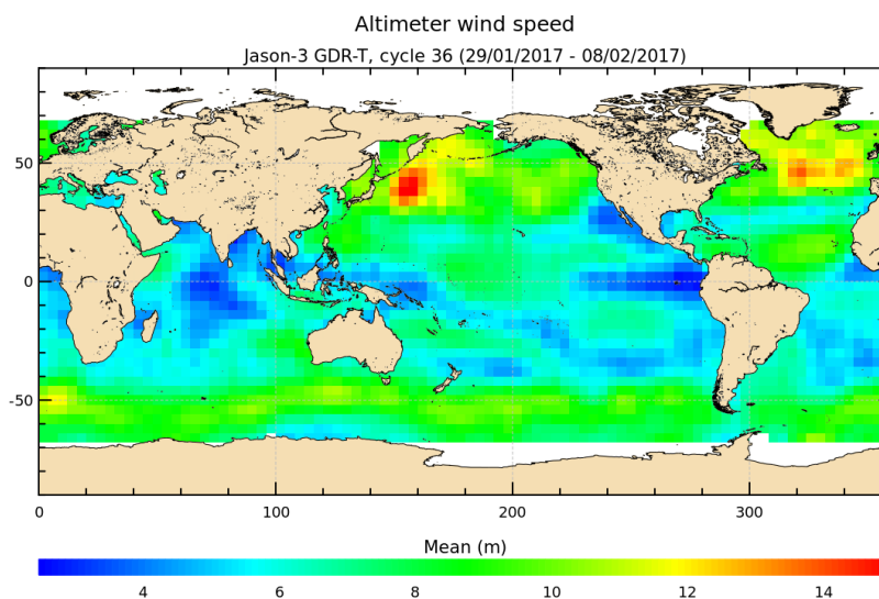
FIGURE 9 – Altimeter wind speed for cycle 036.
