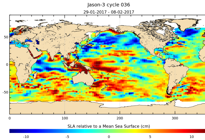
FIGURE 17 – Sea level anomaly relative to MSS for cycle 036.
