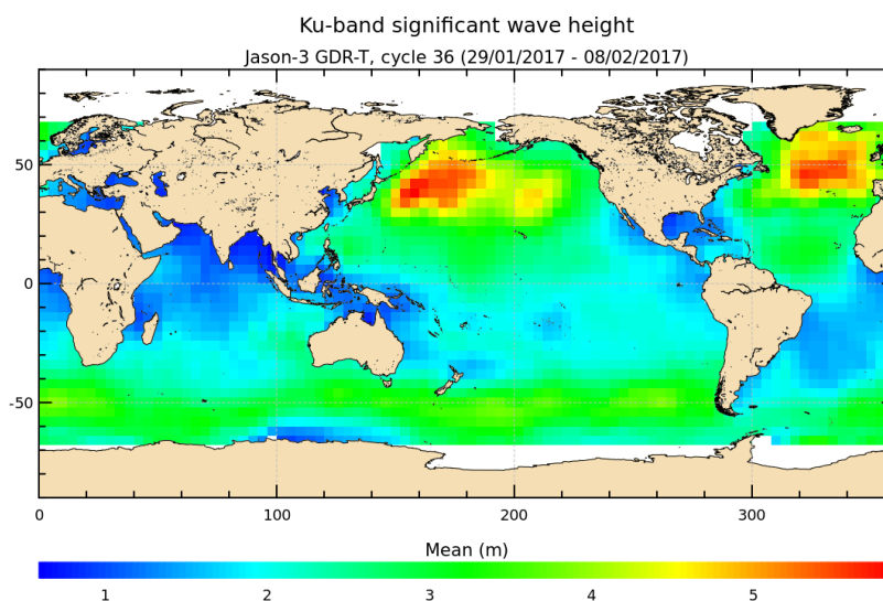
FIGURE 5 – Significant wave height for cycle 036.
