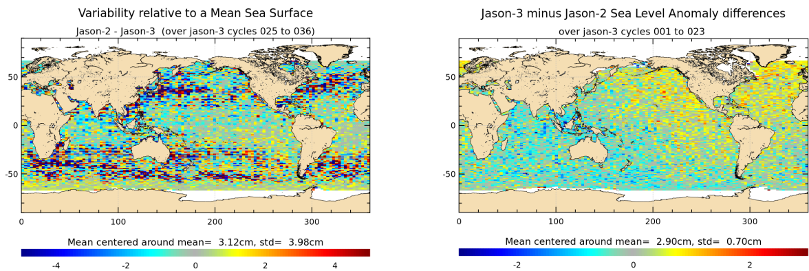
FIGURE 18 – Jason-2 – Jason-3 SLA differences averaged over Jason-3 period from cycle 025 until cycle 036 (left), and for tandem phase (cycle 001 to 023) (right).
