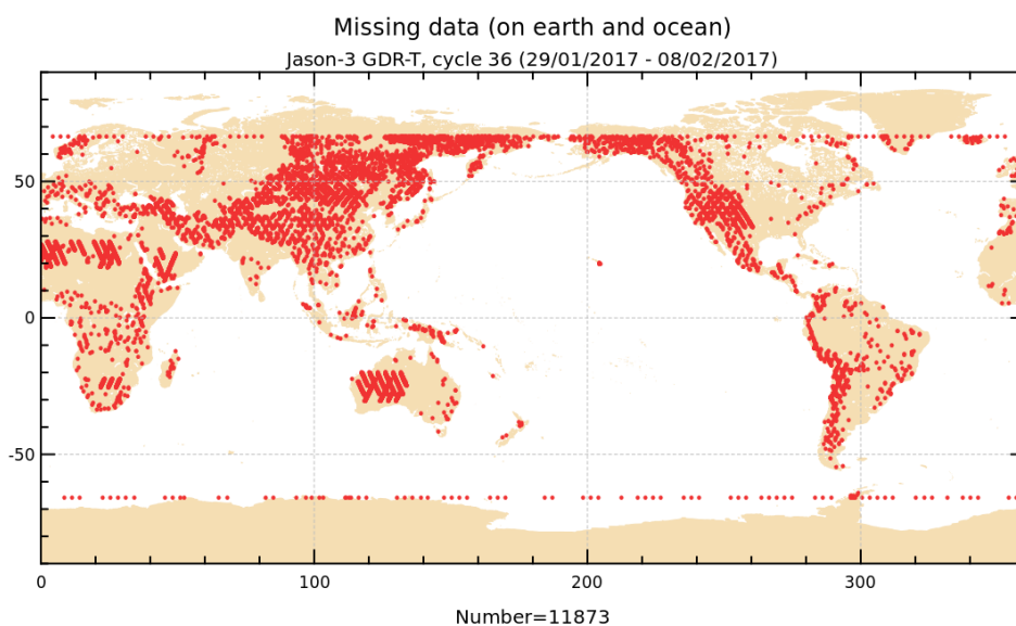
FIGURE 1 – Missing measurements for cycle 036.
