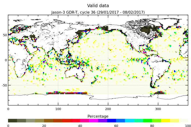
FIGURE 3 – Percentage of valid measurements for cycle 036.
