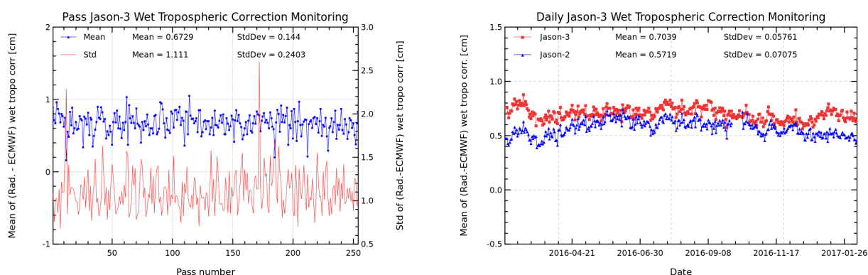
FIGURE 11 – Pass monitoring of wet troposphere differences between radiometer and ECMWF model for Jason-3 cycle 036 (left) and Jason-3 versus Jason-2 daily monitoring of wet troposphere differences between radiometer and ECMWF model (right).
