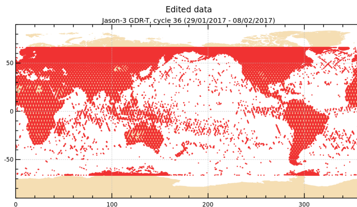
FIGURE 2 – Edited measurements for cycle 036.
