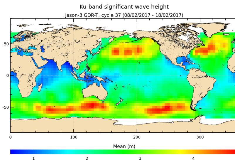
FIGURE 5 – Significant wave height for cycle 037.
