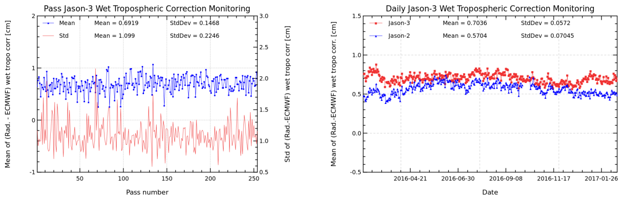
FIGURE 11 – Pass monitoring of wet troposphere differences between radiometer and ECMWF model for Jason-3 cycle 037 (left) and Jason-3 versus Jason-2 daily monitoring of wet troposphere differences between radiometer and ECMWF model (right).
