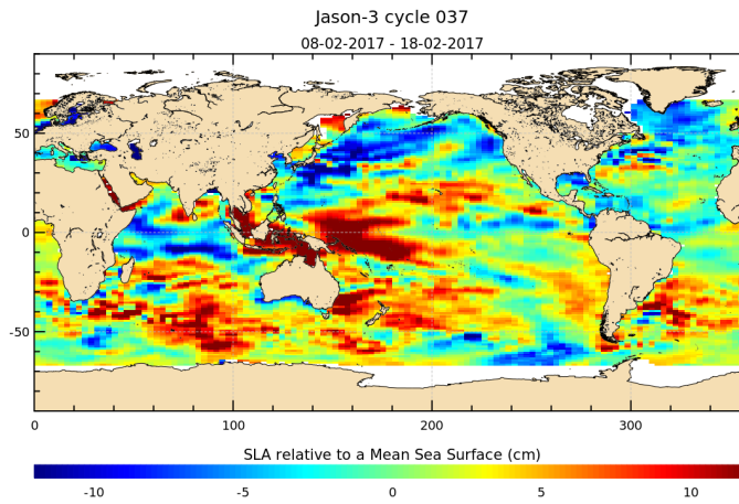
FIGURE 17 – Sea level anomaly relative to MSS for cycle 037.
