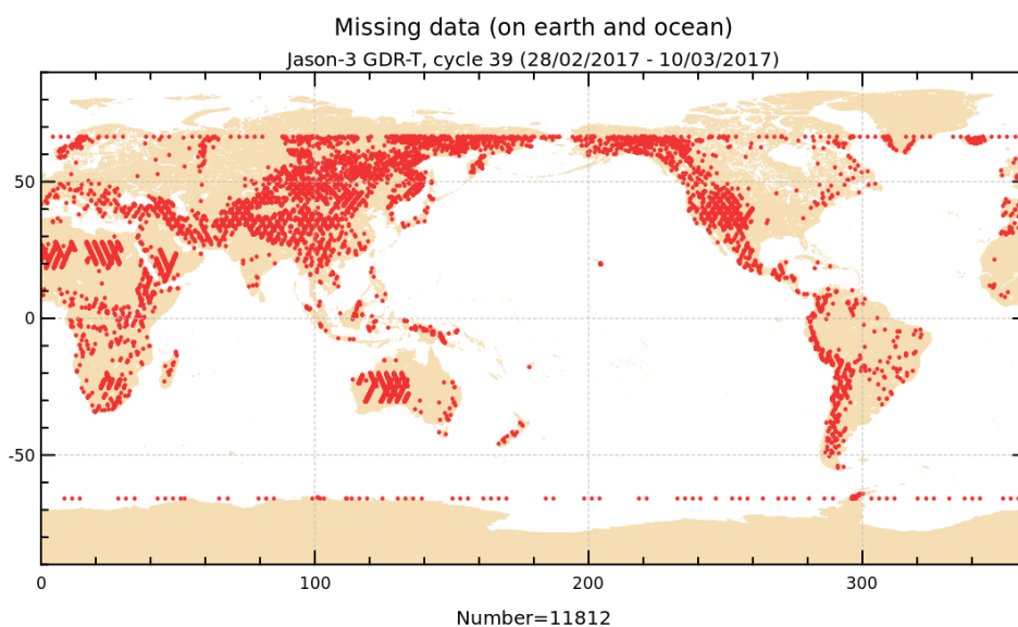
FIGURE 1 – Missing measurements for cycle 039.
