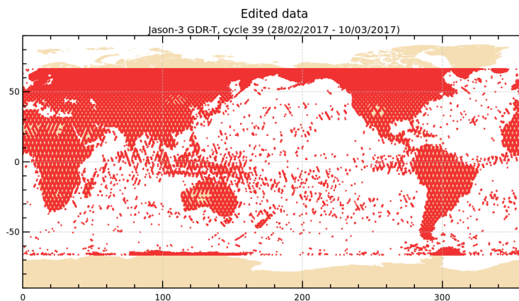
FIGURE 2 – Edited measurements for cycle 039.
