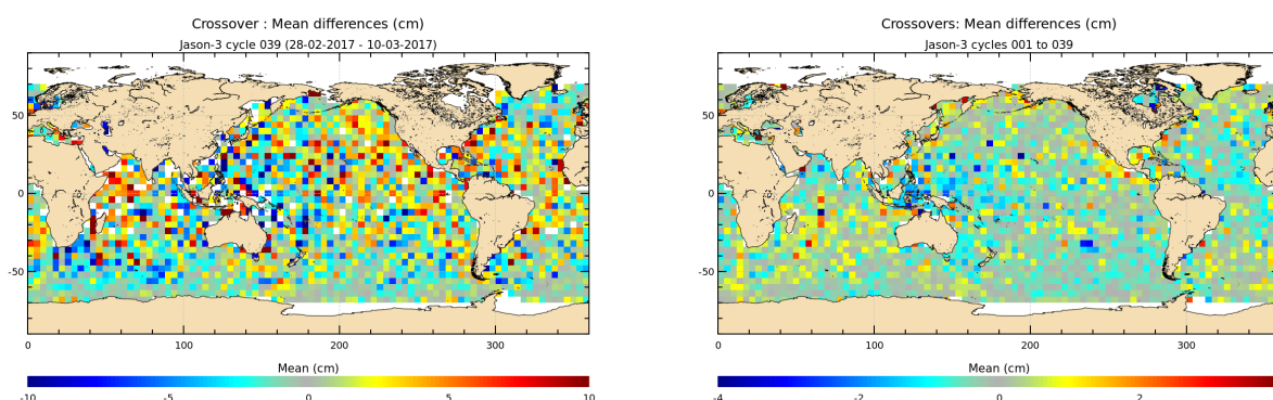
FIGURE 12 – Mean SSH at crossovers for cycle 039 (left) and over the whole Jason-3 period (right).
