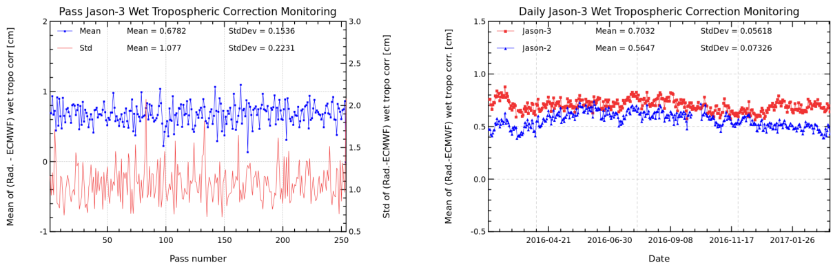
FIGURE 11 – Pass monitoring of wet troposphere differences between radiometer and ECMWF model for Jason-3 cycle 039 (left) and Jason-3 versus Jason-2 daily monitoring of wet troposphere differences between radiometer and ECMWF model (right).
