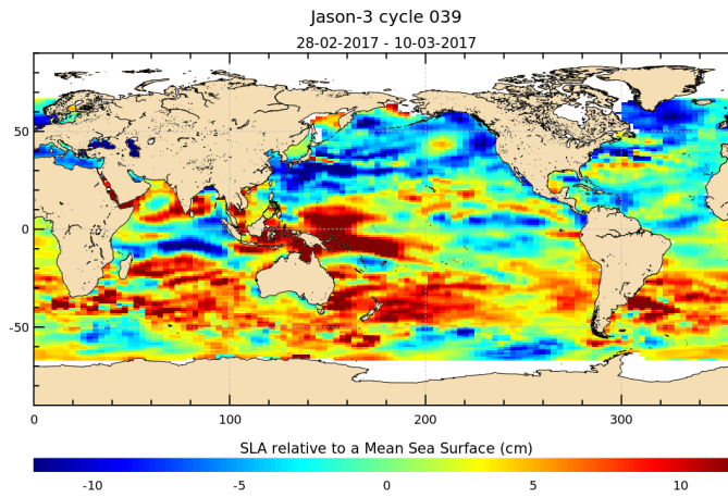
FIGURE 17 – Sea level anomaly relative to MSS for cycle 039.
