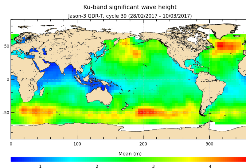
FIGURE 5 – Significant wave height for cycle 039.
