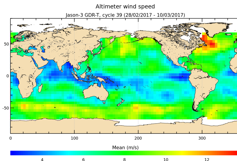
FIGURE 9 – Altimeter wind speed for cycle 039.
