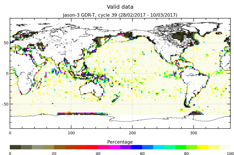
FIGURE 3 – Percentage of valid measurements for cycle 039.
