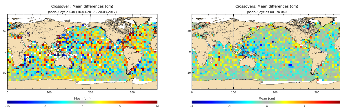
FIGURE 12 – Mean SSH at crossovers for cycle 040 (left) and over the whole Jason-3 period (right).
