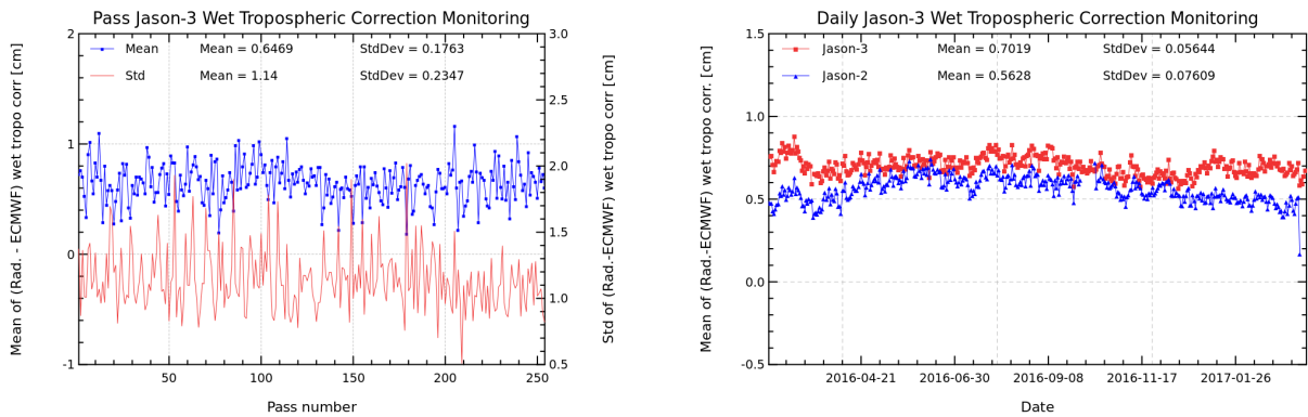
FIGURE 11 – Pass monitoring of wet troposphere differences between radiometer and ECMWF model for Jason-3 cycle 040 (left) and Jason-3 versus Jason-2 daily monitoring of wet troposphere differences between radiometer and ECMWF model (right).
