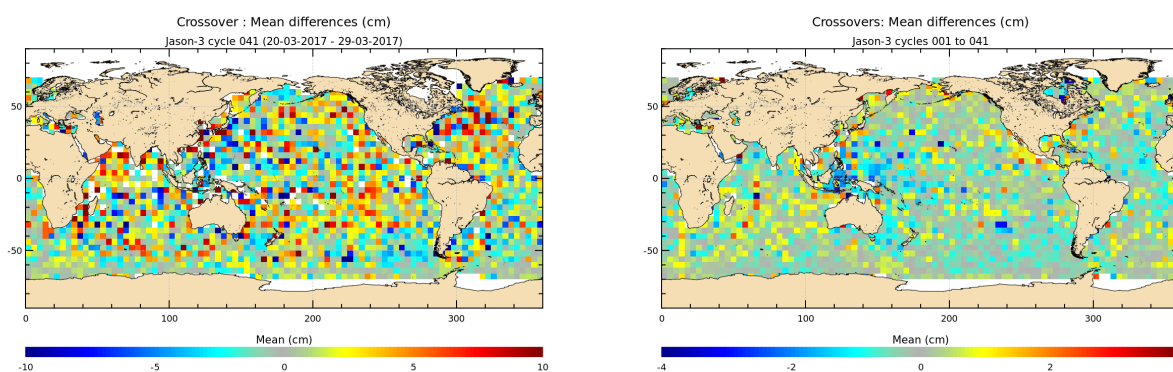
FIGURE 12 – Mean SSH at crossovers for cycle 041 (left) and over the whole Jason-3 period (right).
