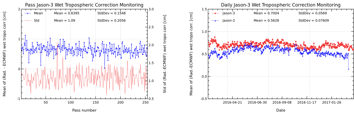
FIGURE 11 – Pass monitoring of wet troposphere differences between radiometer and ECMWF model for Jason-3 cycle 041 (left) and Jason-3 versus Jason-2 daily monitoring of wet troposphere differences between radiometer and ECMWF model (right).
