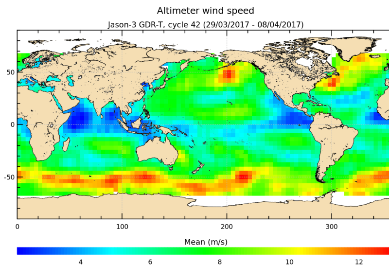
FIGURE 9 – Altimeter wind speed for cycle 042.
