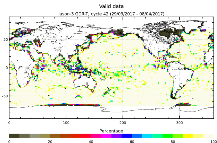
FIGURE 3 – Percentage of valid measurements for cycle 042.
