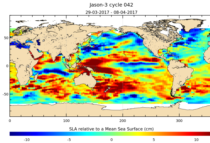
FIGURE 17 – Sea level anomaly relative to MSS for cycle 042.
