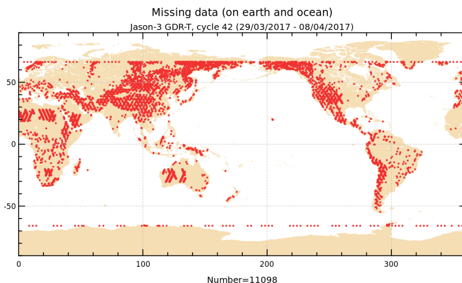
FIGURE 1 – Missing measurements for cycle 042.
