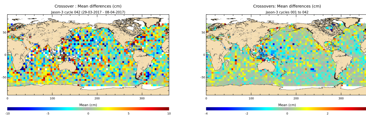
FIGURE 12 – Mean SSH at crossovers for cycle 042 (left) and over the whole Jason-3 period (right).
