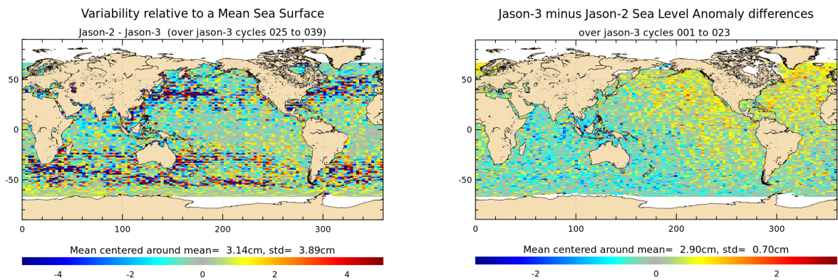
FIGURE 18 – Jason-2 – Jason-3 SLA differences averaged over Jason-3 period from cycle 025 until cycle 039 (left), and for tandem phase (cycle 001 to 023) (right).
