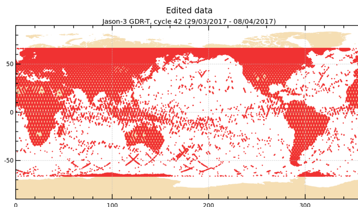
FIGURE 2 – Edited measurements for cycle 042.
