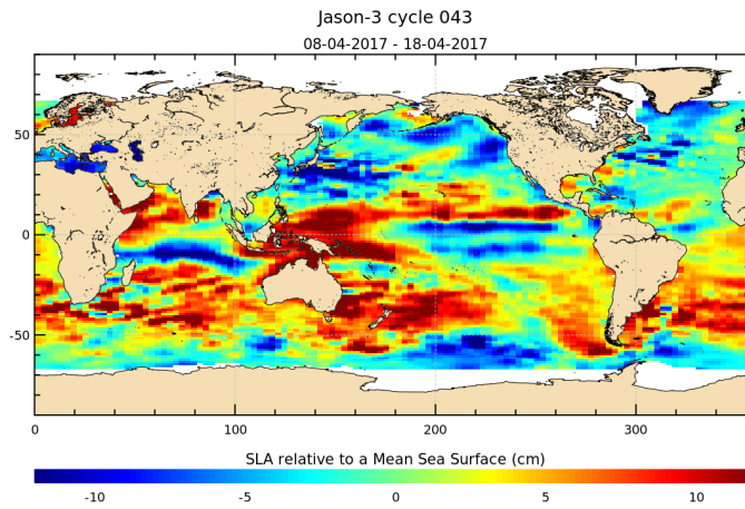
FIGURE 17 – Sea level anomaly relative to MSS for cycle 043.
