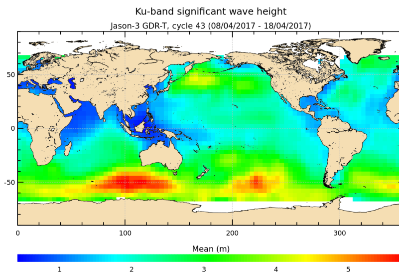
FIGURE 5 – Significant wave height for cycle 043.
