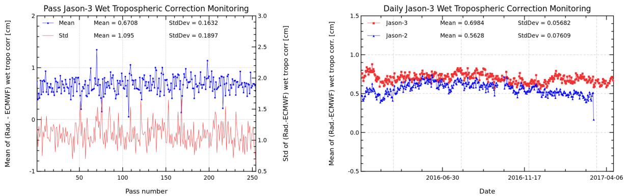
FIGURE 11 – Pass monitoring of wet troposphere differences between radiometer and ECMWF model for Jason-3 cycle 043 (left) and Jason-3 versus Jason-2 daily monitoring of wet troposphere differences between radiometer and ECMWF model (right).
