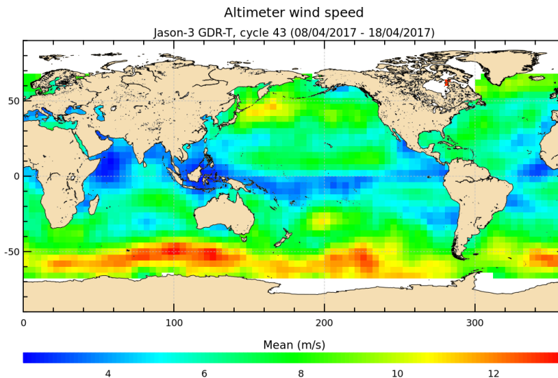
FIGURE 9 – Altimeter wind speed for cycle 043.
