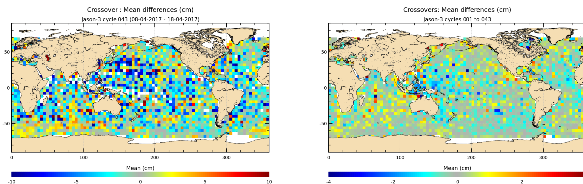
FIGURE 12 – Mean SSH at crossovers for cycle 043 (left) and over the whole Jason-3 period (right).
