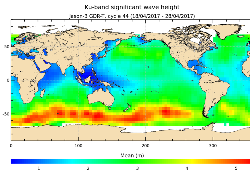
FIGURE 5 – Significant wave height for cycle 044.
