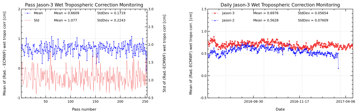
FIGURE 11 – Pass monitoring of wet troposphere differences between radiometer and ECMWF model for Jason-3 cycle 044 (left) and Jason-3 versus Jason-2 daily monitoring of wet troposphere differences between radiometer and ECMWF model (right).
