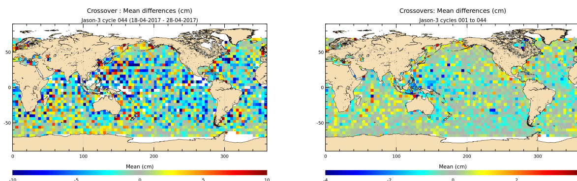
FIGURE 12 – Mean SSH at crossovers for cycle 044 (left) and over the whole Jason-3 period (right).
