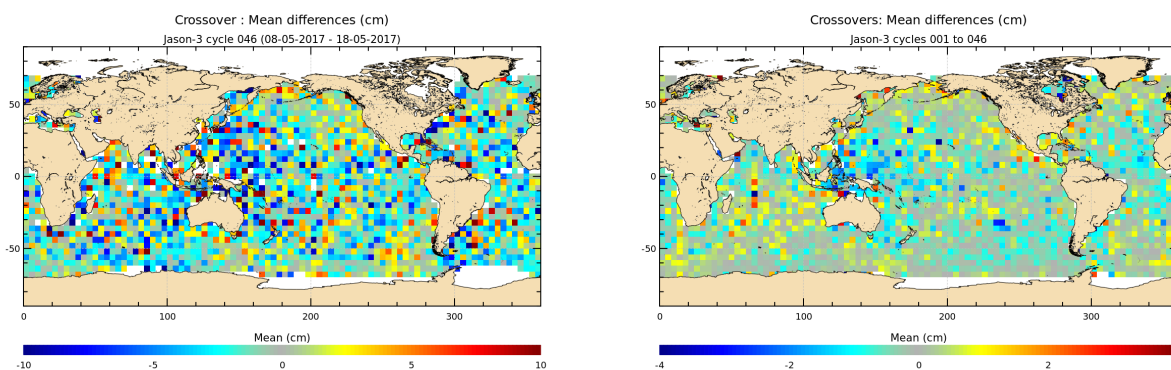
FIGURE 12 – Mean SSH at crossovers for cycle 046 (left) and over the whole Jason-3 period (right).
