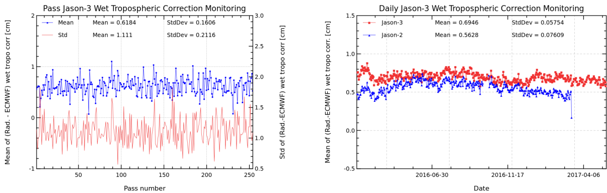
FIGURE 11 – Pass monitoring of wet troposphere differences between radiometer and ECMWF model for Jason-3 cycle 046 (left) and Jason-3 versus Jason-2 daily monitoring of wet troposphere differences between radiometer and ECMWF model (right).
