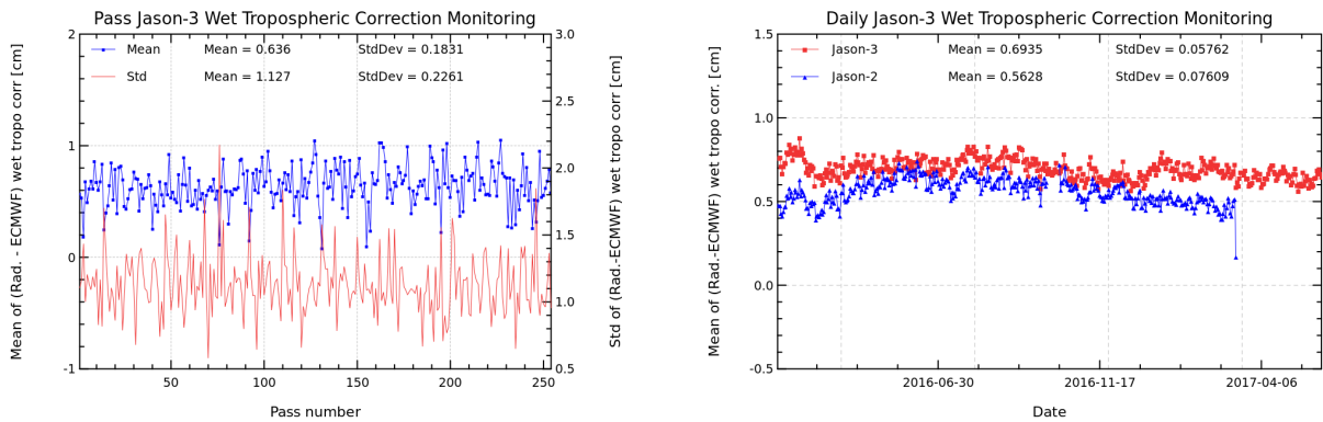
FIGURE 11 – Pass monitoring of wet troposphere differences between radiometer and ECMWF model for Jason-3 cycle 047 (left) and Jason-3 versus Jason-2 daily monitoring of wet troposphere differences between radiometer and ECMWF model (right).
