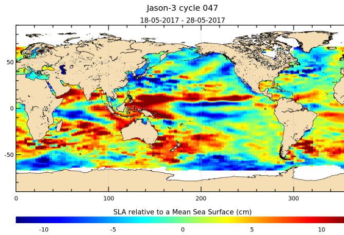
FIGURE 17 – Sea level anomaly relative to MSS for cycle 047.
