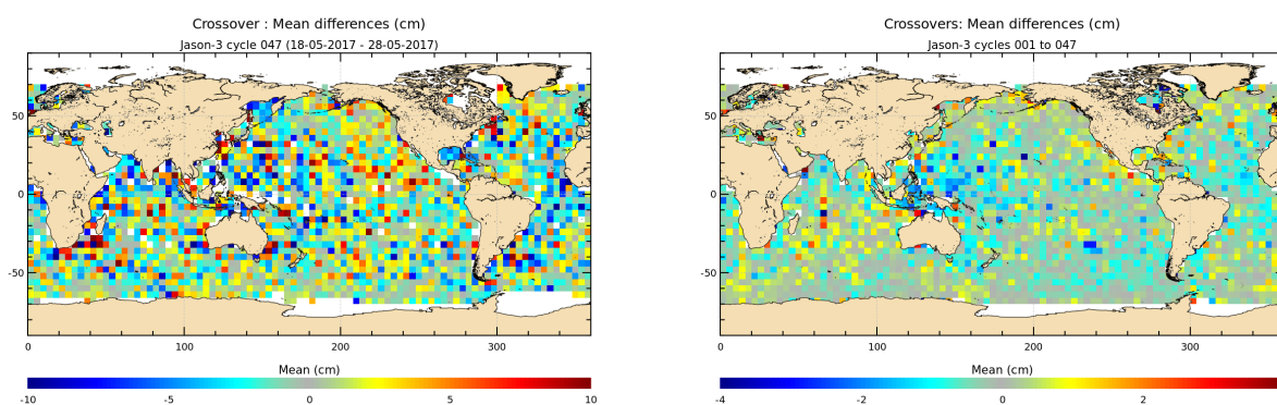
FIGURE 12 – Mean SSH at crossovers for cycle 047 (left) and over the whole Jason-3 period (right).
