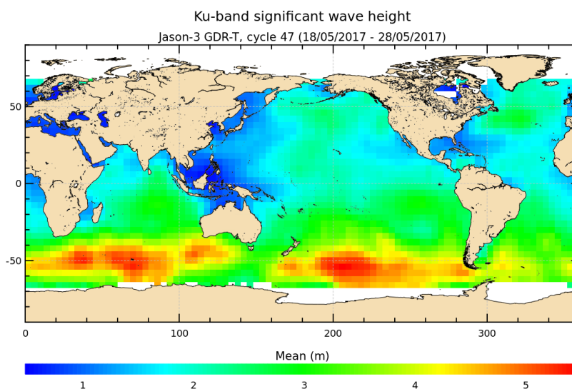
FIGURE 5 – Significant wave height for cycle 047.
