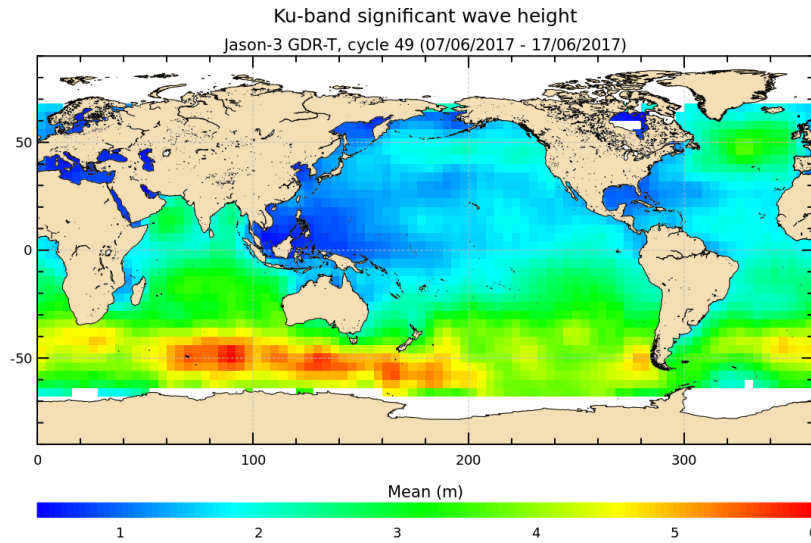
FIGURE 5 – Significant wave height for cycle 049.
