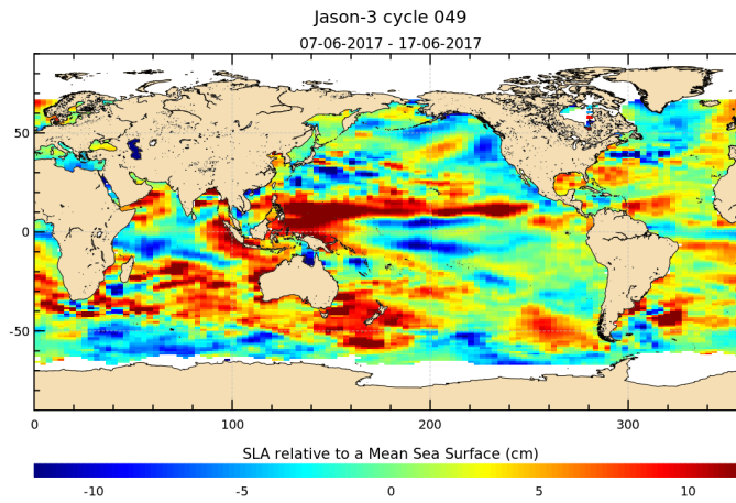
FIGURE 17 – Sea level anomaly relative to MSS for cycle 049.
