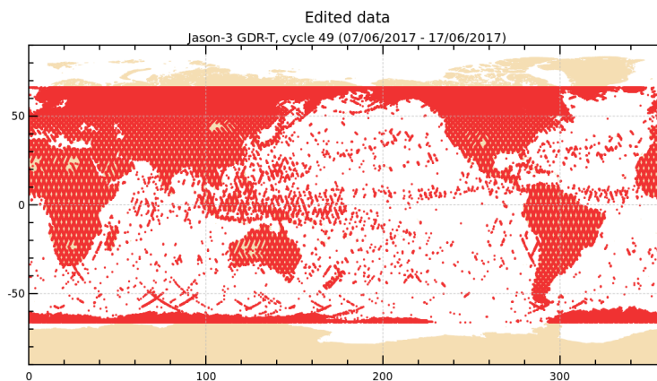
FIGURE 2 – Edited measurements for cycle 049.
