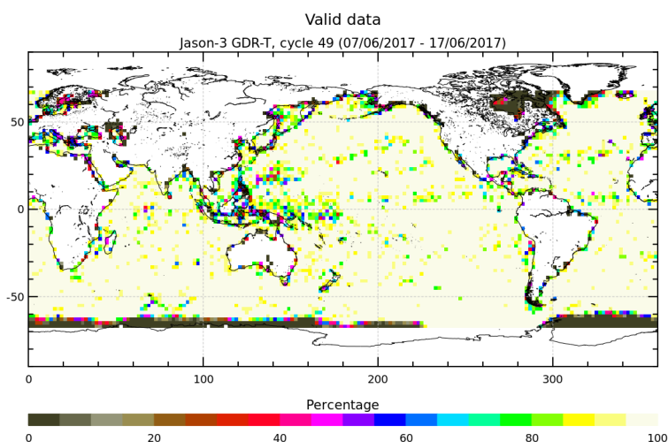
FIGURE 3 – Percentage of valid measurements for cycle 049.
