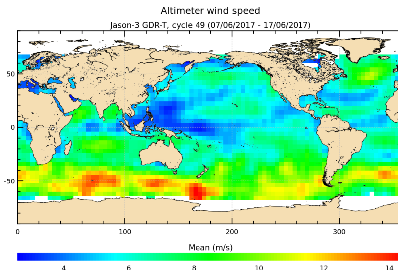
FIGURE 9 – Altimeter wind speed for cycle 049.
