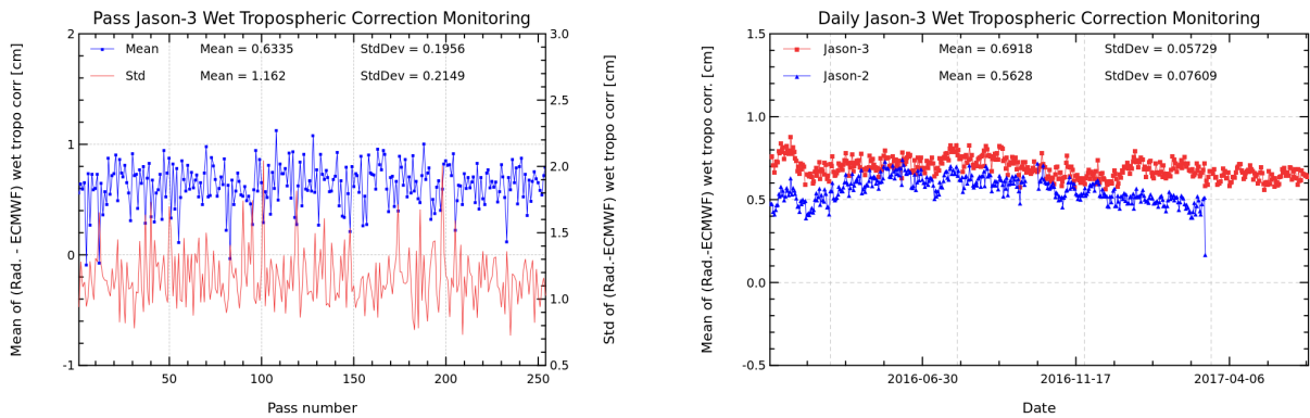
FIGURE 11 – Pass monitoring of wet troposphere differences between radiometer and ECMWF model for Jason-3 cycle 049 (left) and Jason-3 versus Jason-2 daily monitoring of wet troposphere differences between radiometer and ECMWF model (right).
