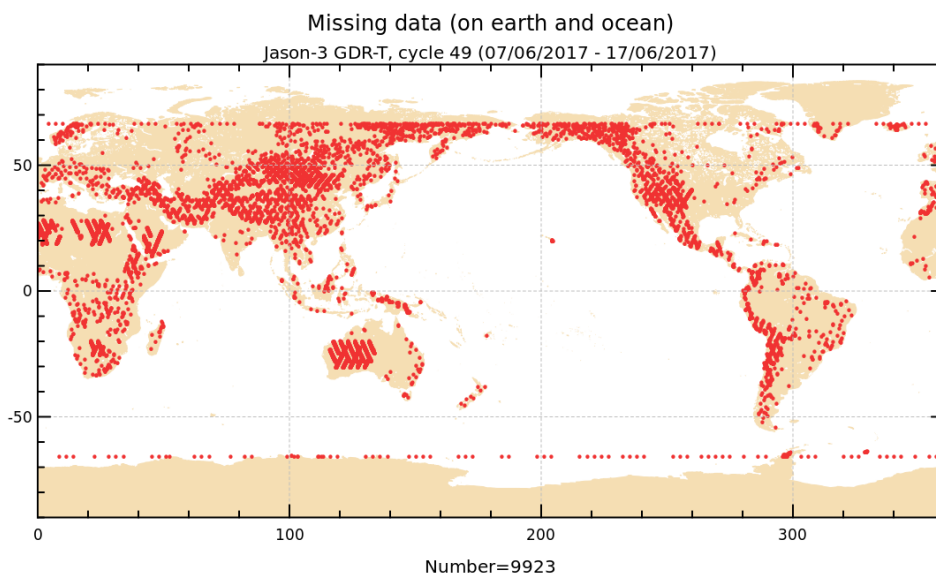
FIGURE 1 – Missing measurements for cycle 049.
