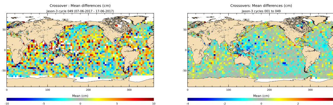
FIGURE 12 – Mean SSH at crossovers for cycle 049 (left) and over the whole Jason-3 period (right).
