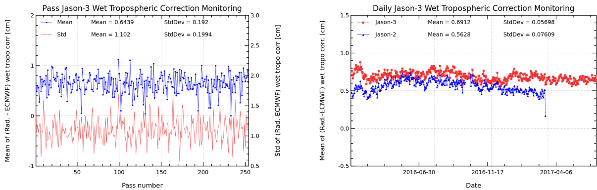
FIGURE 11 – Pass monitoring of wet troposphere differences between radiometer and ECMWF model for Jason-3 cycle 050 (left) and Jason-3 versus Jason-2 daily monitoring of wet troposphere differences between radiometer and ECMWF model (right).
