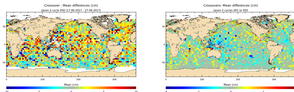
FIGURE 12 – Mean SSH at crossovers for cycle 050 (left) and over the whole Jason-3 period (right).
