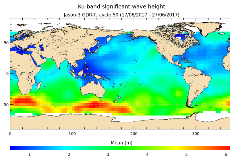
FIGURE 5 – Significant wave height for cycle 050.
