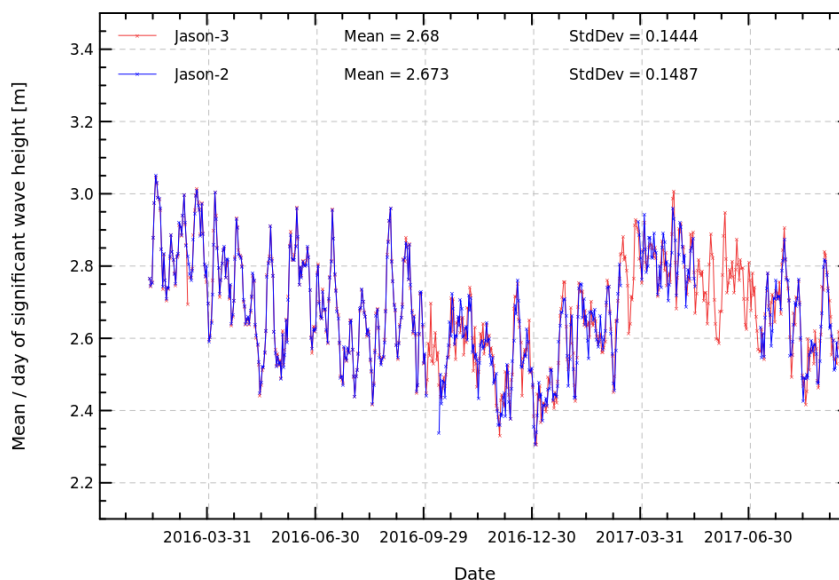
FIGURE 7 – Daily monitoring of Ku-band significant wave height for Jason-2 and Jason-3.
