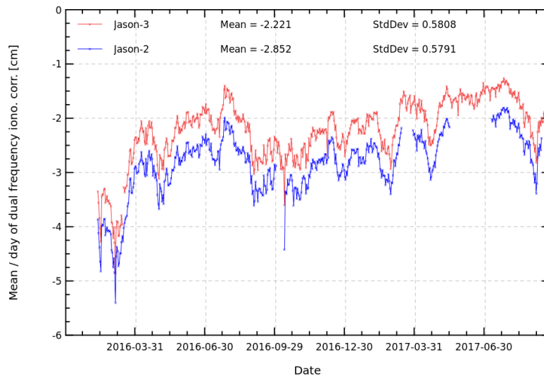
FIGURE 9 – Daily monitoring of dual-frequency ionosphere correction for Jason-2 and Jason-3.
