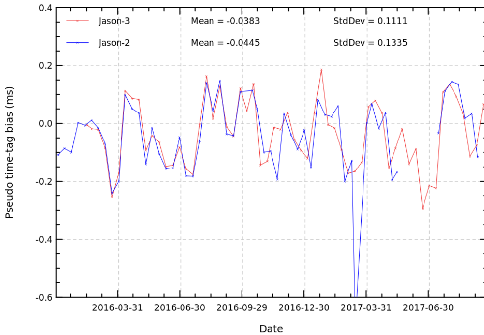
FIGURE 16 – Cyclic monitoring of pseudo time tag bias for Jason-3 and Jason-2.
