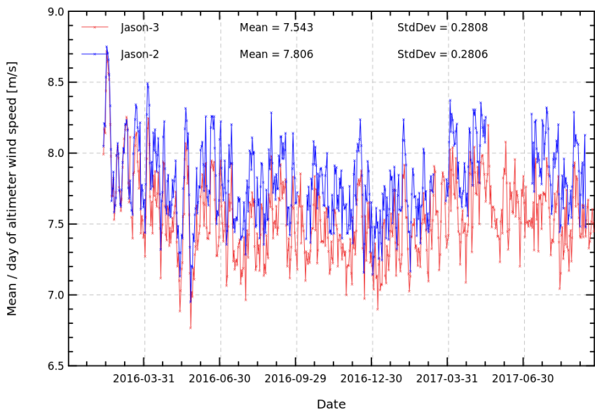
FIGURE 11 – Daily monitoring of altimeter wind speed for Jason-2 and Jason-3.
