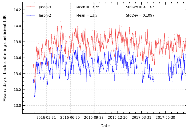
FIGURE 8 – Daily monitoring of Ku-band backscattering coefficient for Jason-2 and Jason-3.
