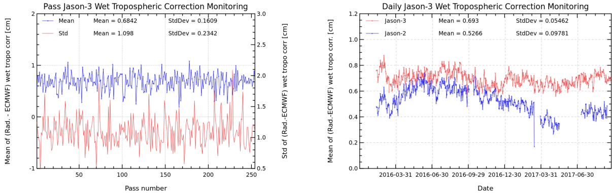
FIGURE 12 – Pass monitoring of wet troposphere differences between radiometer and ECMWF model for Jason-3 cycle 059 (left) and Jason-3 versus Jason-2 daily monitoring of wet troposphere differences between radiometer and ECMWF model (right).
