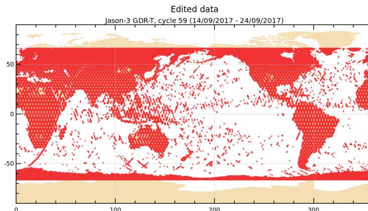
FIGURE 2 – Edited measurements for cycle 059.
