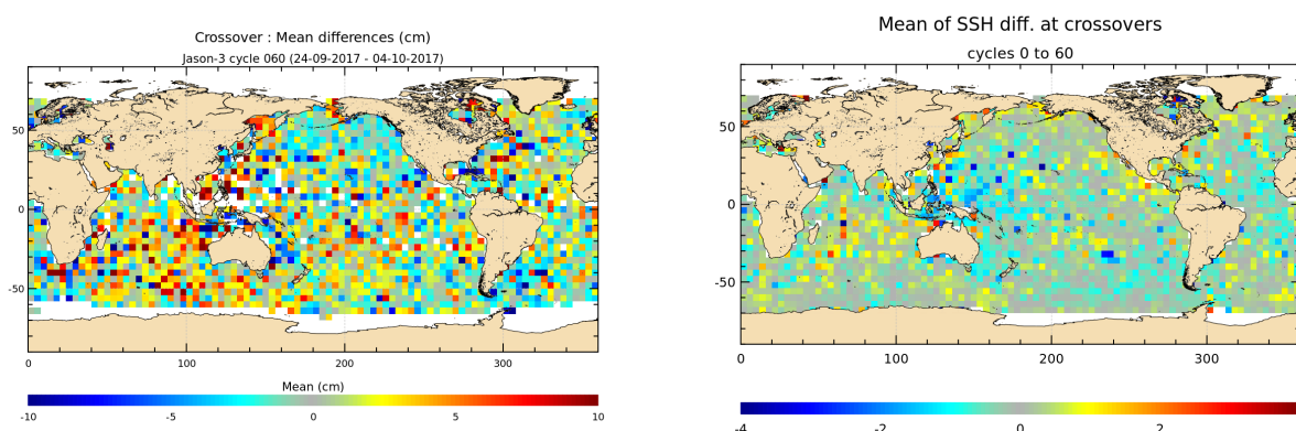
FIGURE 12 – Mean SSH at crossovers for cycle 060 (left) and over the whole Jason-3 period (right).
