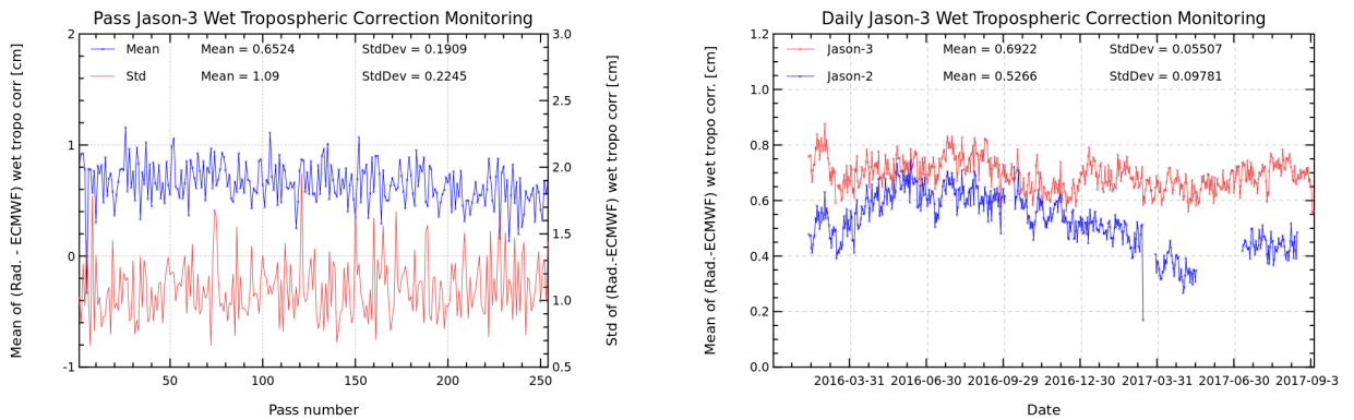
FIGURE 11 – Pass monitoring of wet troposphere differences between radiometer and ECMWF model for Jason-3 cycle 060 (left) and Jason-3 versus Jason-2 daily monitoring of wet troposphere differences between radiometer and ECMWF model (right).
