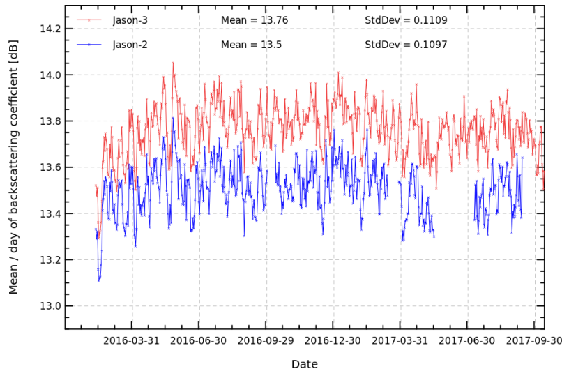
FIGURE 7 – Daily monitoring of Ku-band backscattering coefficient for Jason-2 and Jason-3.
