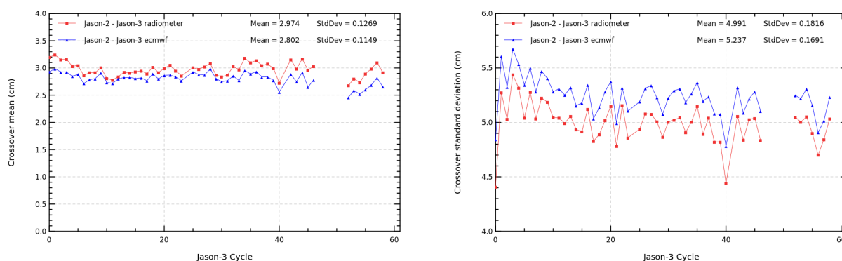
FIGURE 14 – Cyclic monitoring of mean (left) and standard deviation (right) of (Jason-2 – Jason-3) SSH differences at crossovers.
