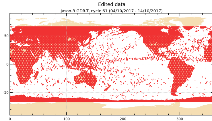
FIGURE 2 – Edited measurements for cycle 061.
