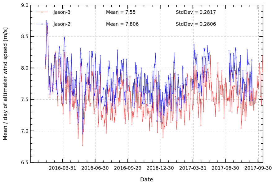
FIGURE 10 – Daily monitoring of altimeter wind speed for Jason-2 and Jason-3.
