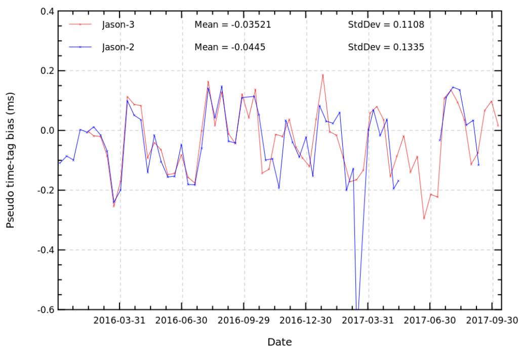
FIGURE 15 – Cyclic monitoring of pseudo time tag bias for Jason-3 and Jason-2.
