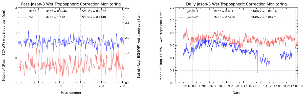
FIGURE 11 – Pass monitoring of wet troposphere differences between radiometer and ECMWF model for Jason-3 cycle 061 (left) and Jason-3 versus Jason-2 daily monitoring of wet troposphere differences between radiometer and ECMWF model (right).
