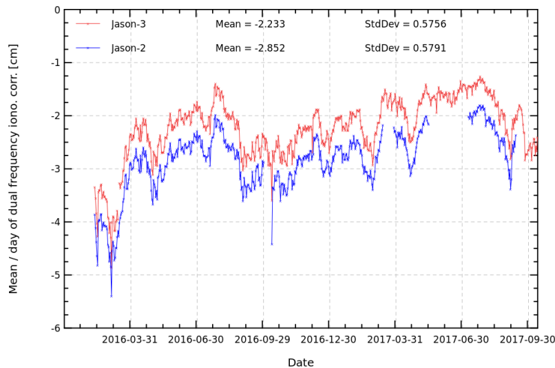
FIGURE 8 – Daily monitoring of dual-frequency ionosphere correction for Jason-2 and Jason-3.
