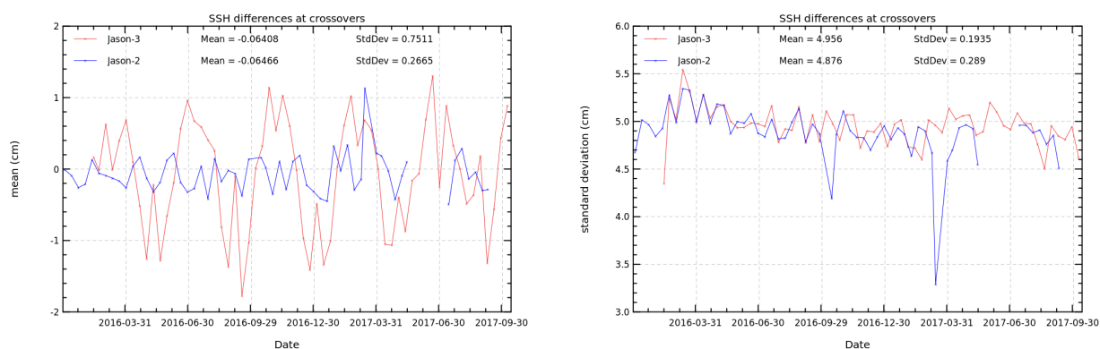
FIGURE 13 – Cyclic monitoring of mean (left) and standard deviation (right) of SSH differences at crossovers for Jason-3 and Jason-2.
