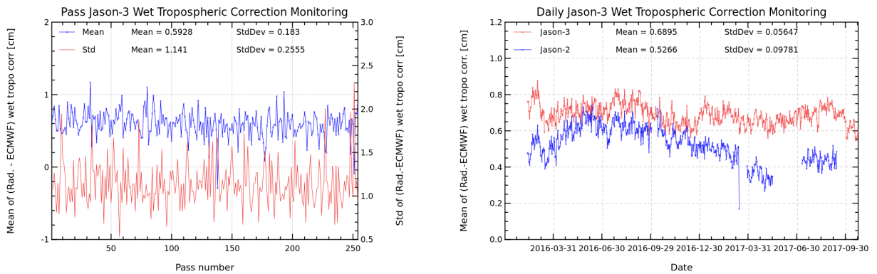
FIGURE 11 – Pass monitoring of wet troposphere differences between radiometer and ECMWF model for Jason-3 cycle 062 (left) and Jason-3 versus Jason-2 daily monitoring of wet troposphere differences between radiometer and ECMWF model (right).
