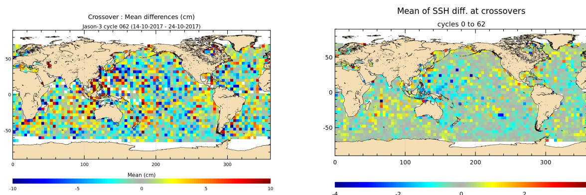
FIGURE 12 – Mean SSH at crossovers for cycle 062 (left) and over the whole Jason-3 period (right).
