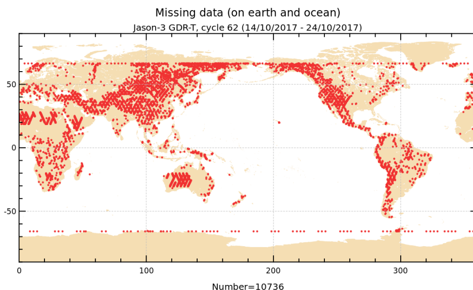
FIGURE 1 – Missing measurements for cycle 062.
