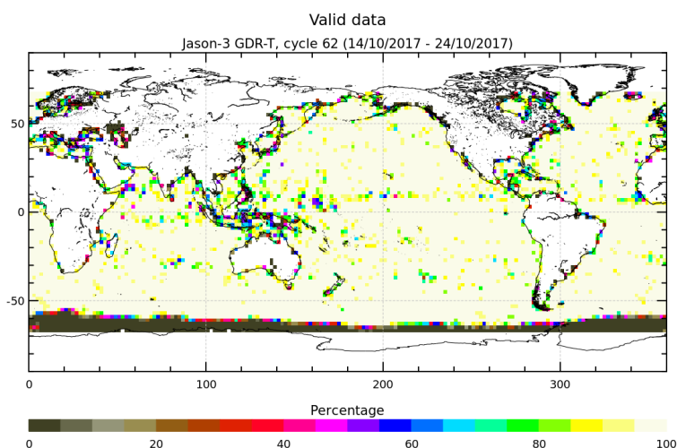
FIGURE 3 – Percentage of valid measurements for cycle 062.
