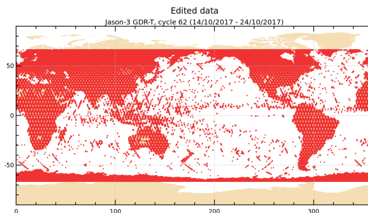
FIGURE 2 – Edited measurements for cycle 062.
