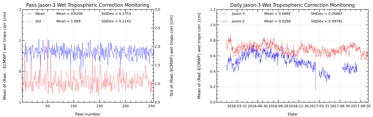
FIGURE 11 – Pass monitoring of wet troposphere differences between radiometer and ECMWF model for Jason-3 cycle 063 (left) and Jason-3 versus Jason-2 daily monitoring of wet troposphere differences between radiometer and ECMWF model (right).
