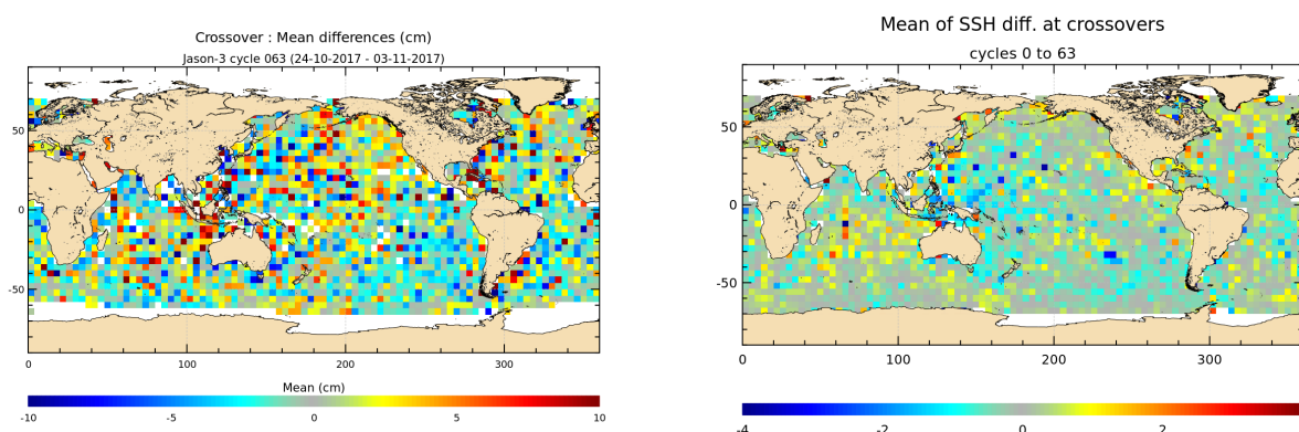
FIGURE 12 – Mean SSH at crossovers for cycle 063 (left) and over the whole Jason-3 period (right).
