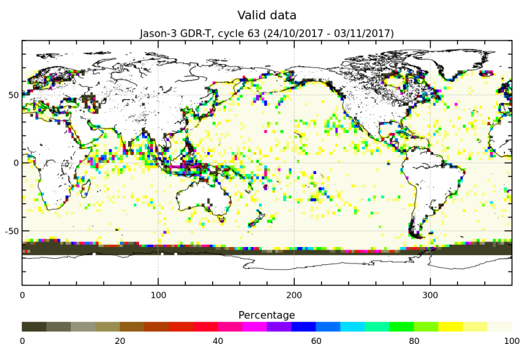
FIGURE 3 – Percentage of valid measurements for cycle 063.
