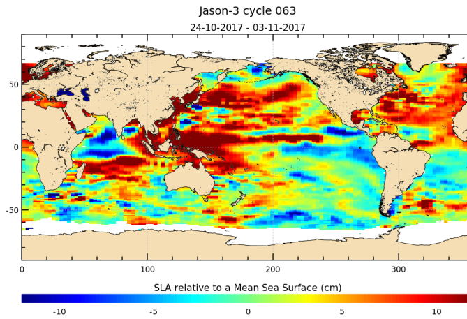
FIGURE 17 – Sea level anomaly relative to MSS for cycle 063.
