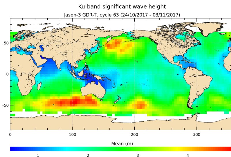
FIGURE 5 – Significant wave height for cycle 063.
