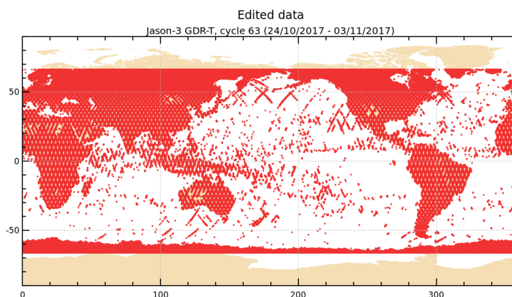
FIGURE 2 – Edited measurements for cycle 063.
