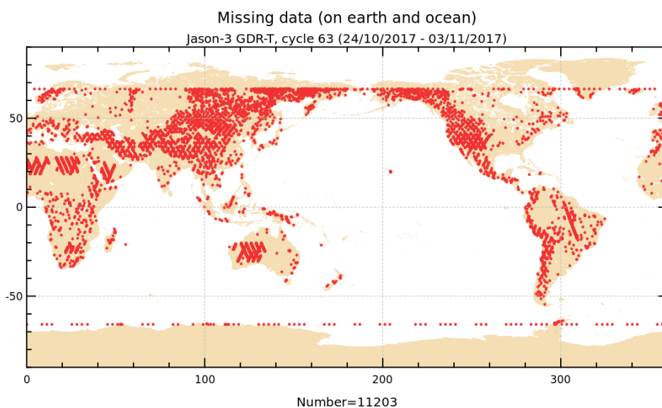
FIGURE 1 – Missing measurements for cycle 063.
