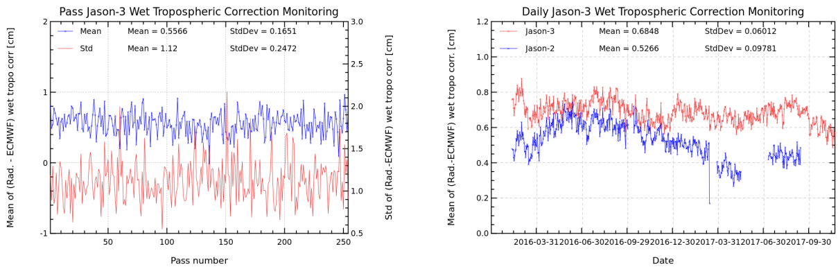
FIGURE 11 – Pass monitoring of wet troposphere differences between radiometer and ECMWF model for Jason-3 cycle 065 (left) and Jason-3 versus Jason-2 daily monitoring of wet troposphere differences between radiometer and ECMWF model (right).
