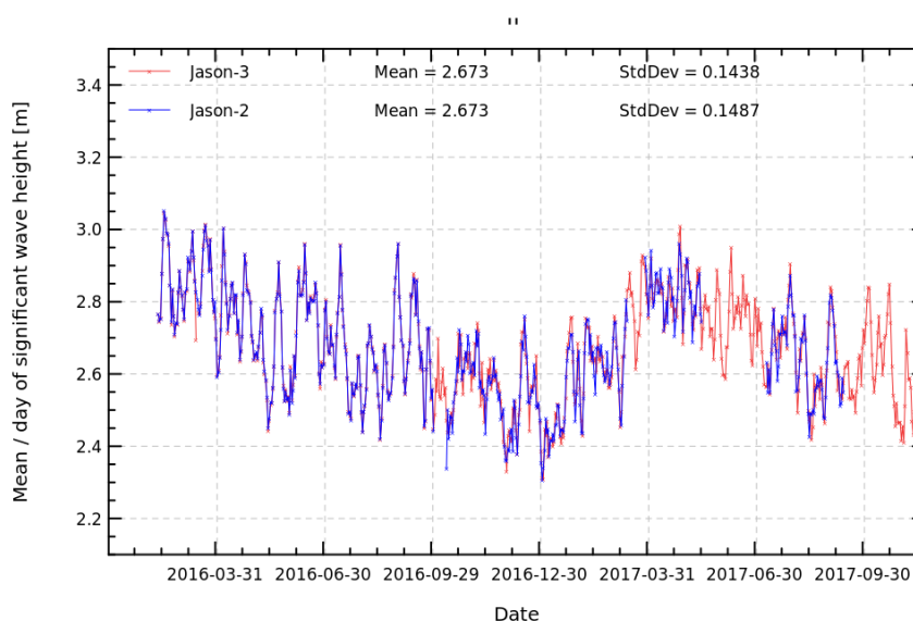
FIGURE 6 – Daily monitoring of Ku-band significant wave height for Jason-2 and Jason-3.
