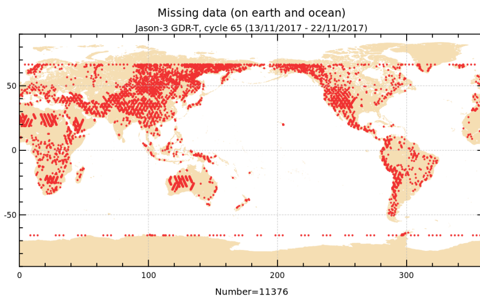
FIGURE 1 – Missing measurements for cycle 065.
